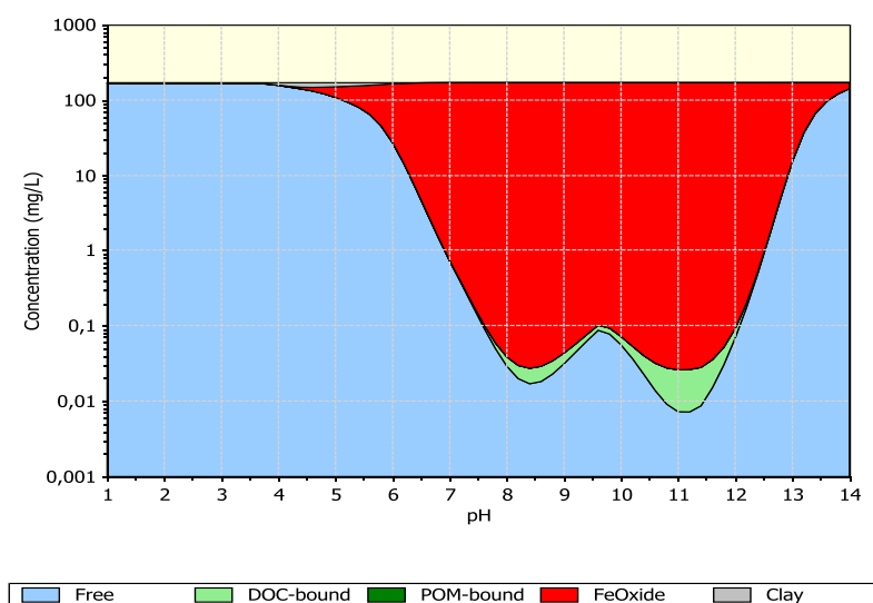
Figure 9: Speciation of Zn in spent MBR and in solution (Free = Zn in solution, DOC-bound = Zn complexed by dissolved organic carbon in solution, POM-bound = Zn complexed by particulate organic matter, FeOxide = Zn adsorbed/complexed by reactive Fe and Al oxihydroxides, Clay = Zn non-specific adsorbed on clay)
