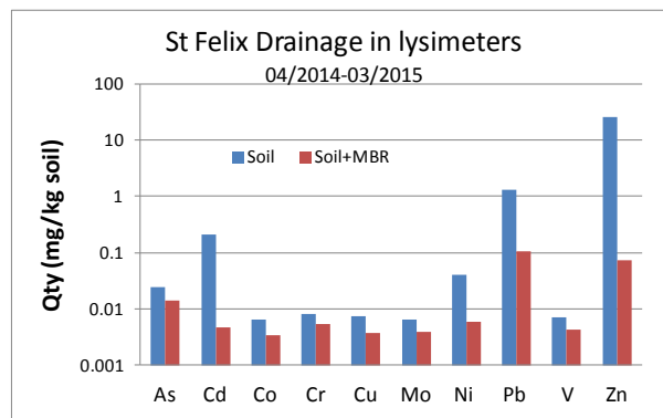
Figure 2: Cumulative emission of trace elements of a pyritic mining residue not treated (soil) and treated (soil + MBR) in lysimeters during one year
