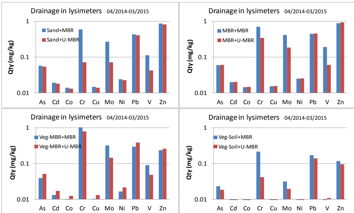
Figure 8: Emission of trace elements from MBR not used for water treatment (MBR) and after water treatment (U-MBR), with different top layer (sand, MBR, vegetated MBR, and vegetated soil).
