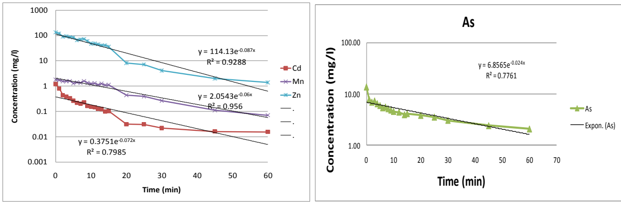
Figure 4: Kinetic of immobilisation for some elements
