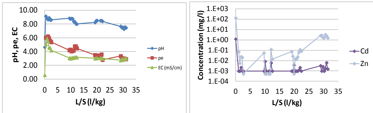
Figure 6: pH, redox potential (pe) and electric conductivity of the water at the outlet of the pilot, and concentration of Cd and Zn at the outlet of the pilot (initial concentration 132 mg Zn/l and 1.21 mg Cd/l).
