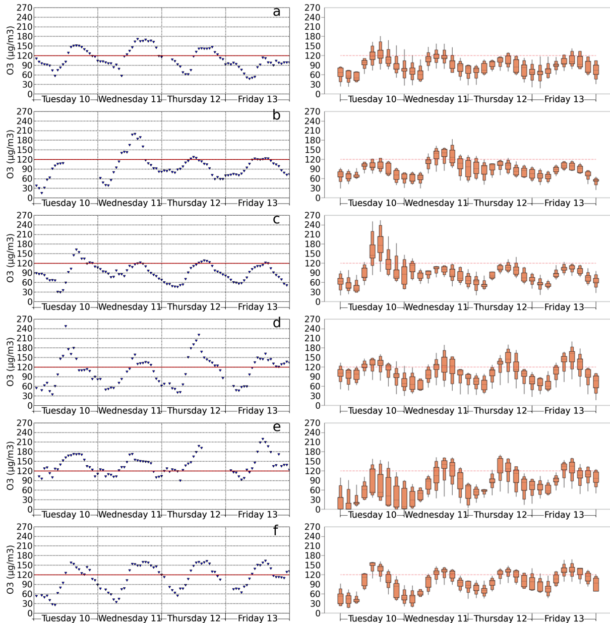
Figure 3. Left panels: ozone measurements from surface stations (in \mu\text{g m}^{-3} ) from 10 June 2014 at 00:00 UTC to 14 June 2014 at 00:00 UTC, located at (a) 47.67° N, 13.11° E (Hallein, Austria), (b) 47.69° N, 16.58° E (Sopron, Hungary), (c) 50.13° N, 8.75° E (Fechenheim, Germany), (d) 43.33° N, 5.12° E (Sausset, France), (e) 43.34° N, 5.73° E (Plan d'Aups, France) and (f) 43.79° N, 4.83° E (St Rémi, France). Right panels: EPSgrams giving median, 90th percentile, 75th percentile, 25th percentile, 10th percentile, minimum and maximum from 3 h outputs of the 96 h forecasts of the seven models from 10 June 2014 at 00:00 UTC to 14 June 2014 at 00:00 UTC. Model outputs are interpolated at the location of the stations shown in the left panel. The red dashed line corresponds to 120 \mu\text{g m}^{-3} .
