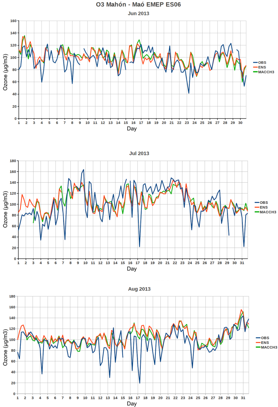
Figure 11. As Fig. 10 but for Mahón (39.867° N, 4.32° W).
