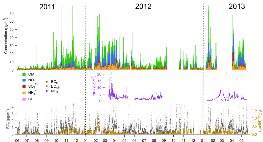
Figure 1. Time series of the major 30 min non-refractory (top, concentrations are aggregated) and 5 min refractory (bottom, concentrations are dissociated) PM 1 chemical constituents, and 5 min ammonia at SIRTa from June 2011 to May 2013. The two large data gaps in October 2012 and March 2013 correspond to two field intensive campaigns during which the ACSM was deployed elsewhere.
