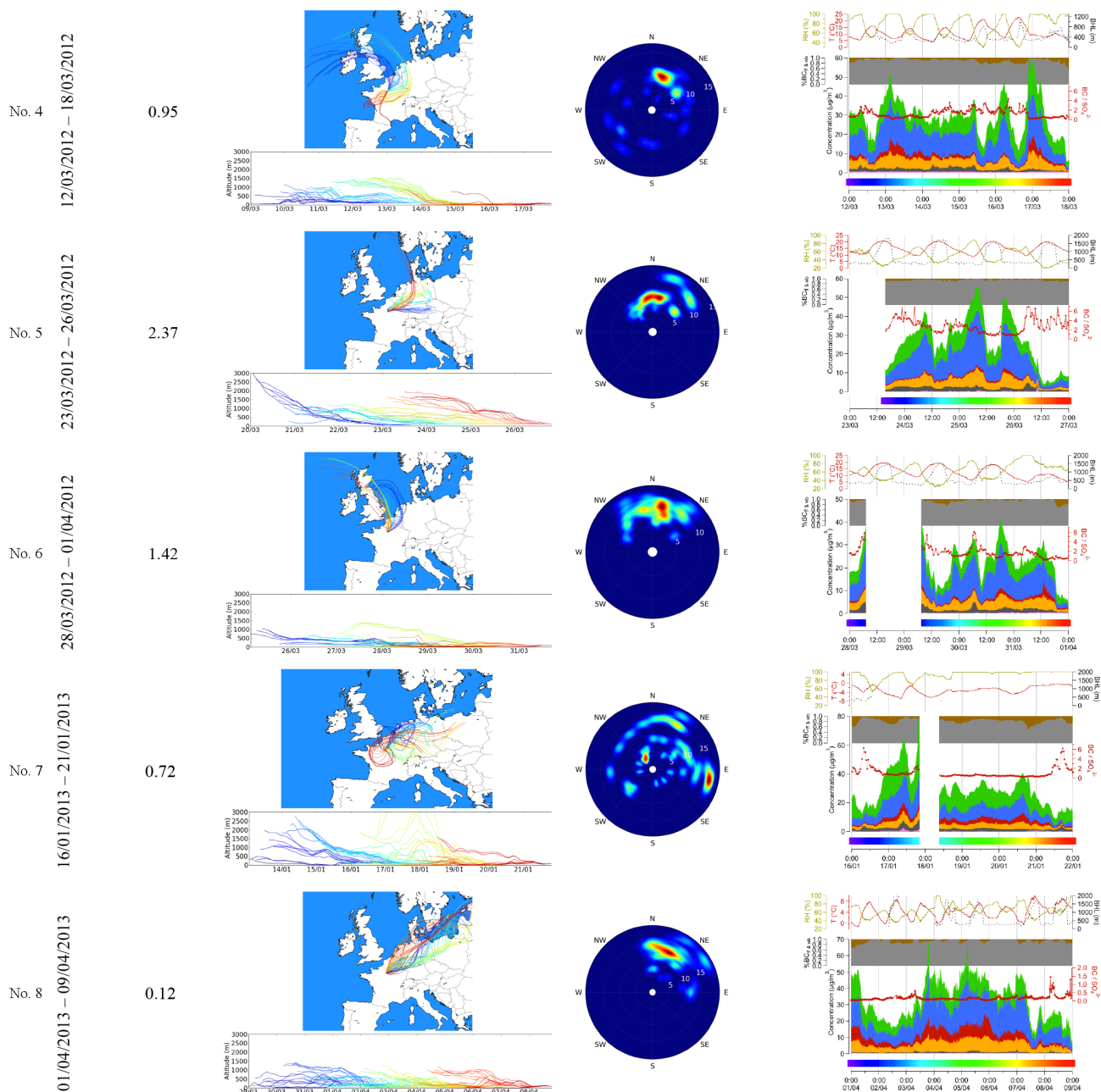
Figure 13. Illustration of meteorological conditions and chemical composition during the eight pollution episodes. Left graphs represent 72 h backtrajectories ending at SIRTa at 100 m a.g.l. every 3 h and their altitude; middle graphs illustrate the wind rose (radial axis in \text{km h}^{-1} ); right graphs represent the chemical composition, in \mu\text{g m}^{-3} of submicron particles (organic, nitrate, sulfate, ammonium, chloride and black carbon in green, blue, red, orange, pink and dark grey, respectively), the contribution of traffic and wood burning to BC, the \text{BC} / \text{SO}_4^{2-} ratio, and temperature, RH and BLH.
