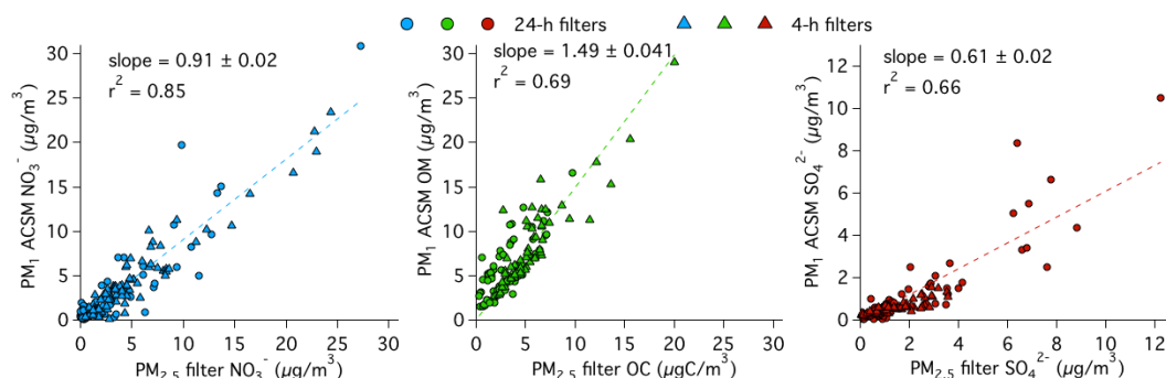
Figure 2. Scatterplot of chemically speciated ACSM measurements versus filter analyses for nitrate, organic matter (compared to OC filter-based measurements) and sulfate.
