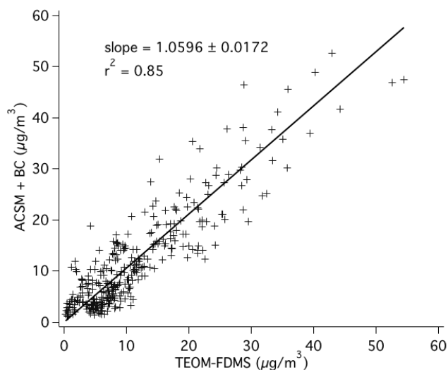
Figure 3. Mass closure exercise between daily averaged reconstructed \text{PM}_{10} (ACSM + BC) and measured \text{PM}_{10} by TEOM-FDMS.
