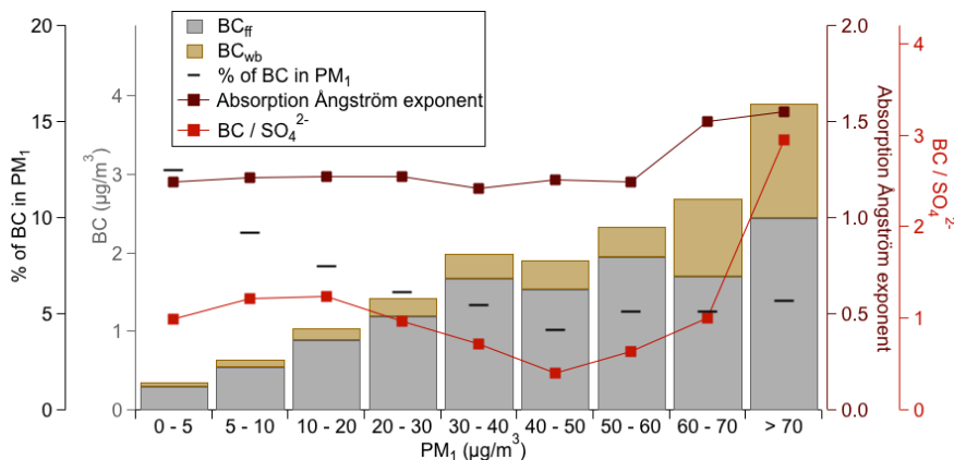
Figure 7. Source contribution to BC, absorption Ångström exponent, BC/SO 4 ratio (ACSM sulfate), and contribution of BC to PM 1 , depending on PM 1 mass.
