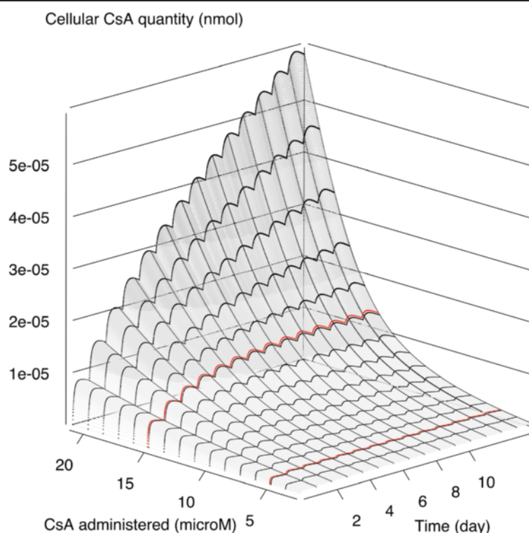
Figure 3 Predictions of RPTECs intracellular CsA quantity versus time and dose during repeated dosing. Thick red lines are predictions for 5 \mu M and 15 \mu M dosing.
