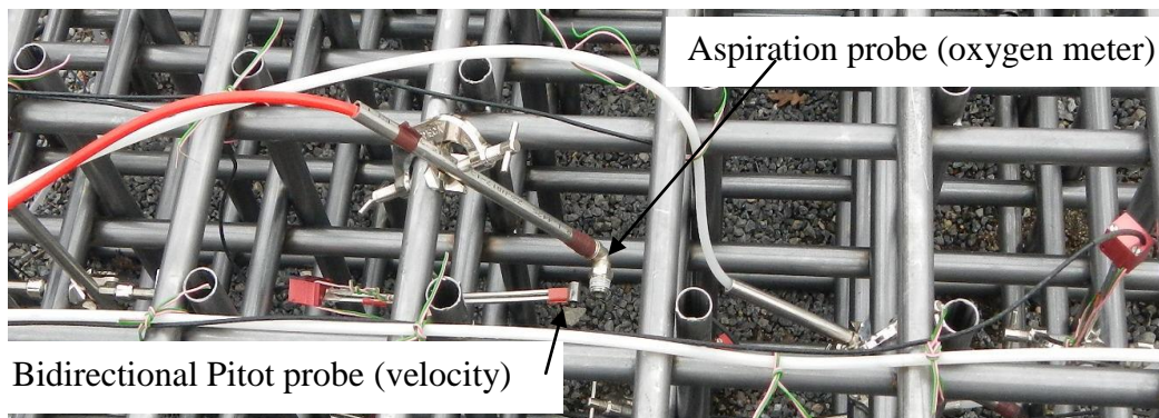
Figure 17 : aspiration probes and bidirectional Pitot probes used for the dispersion tests with the medium congestion module
