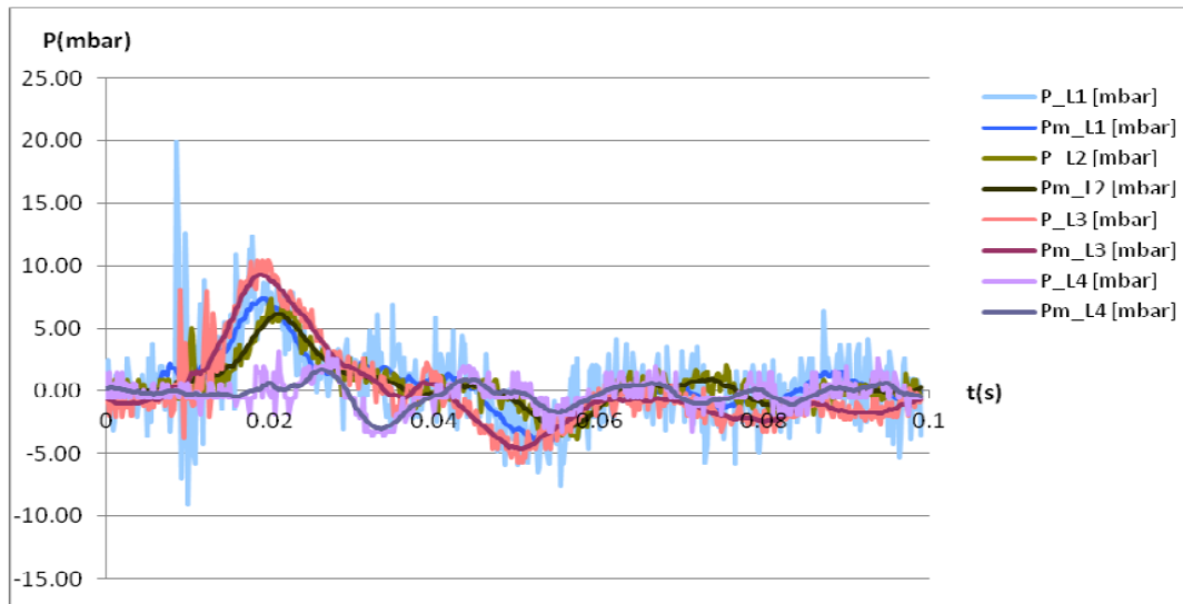
Figure 7 : overpressure signals for 1 test of free jet
