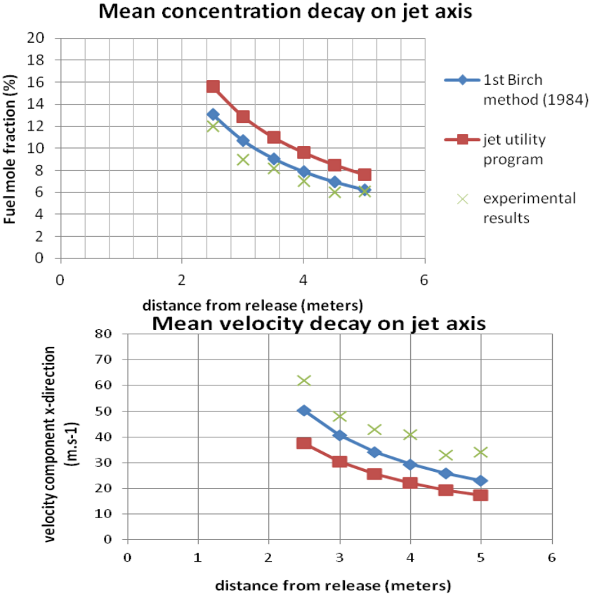
Figure 10 : centreline axial concentration (top) and axial mean velocity(bottom) decays estimated with FLACS using 2 pseudo-source methods. Compared to experimental measures (GDF SUEZ/INERIS tests, 2011-2013)
