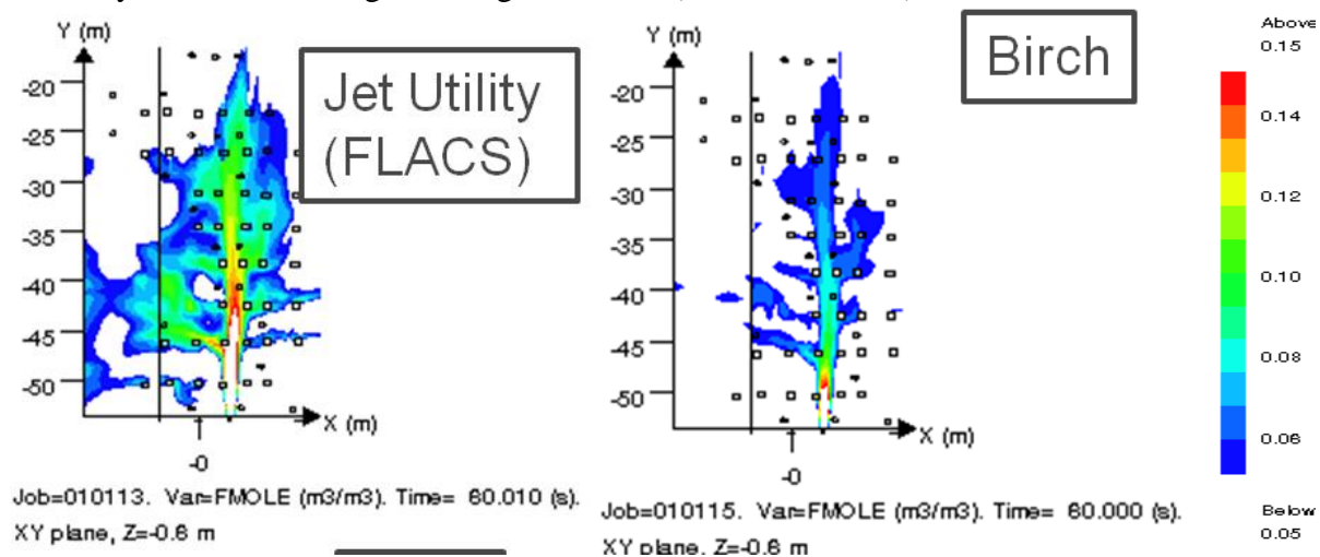
Figure 19 : comparisons of mean concentration fields for different source-term methods.
