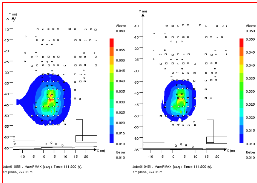
Figure 21 : dispersion calculation: comparisons of mean concentration fields for different
