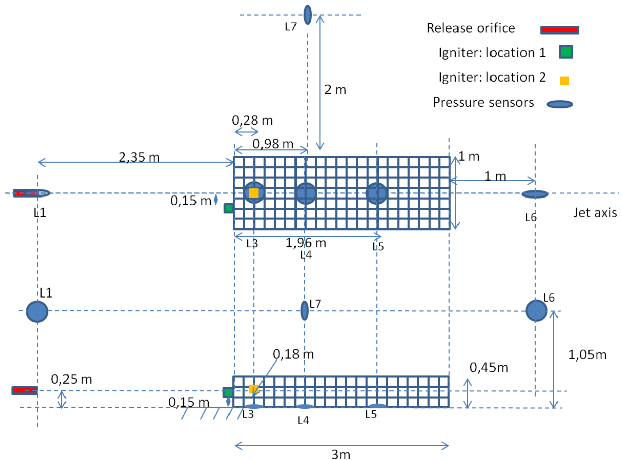
Figure 15 : locations of the release orifice, pipes, igniter and pressure sensors used by INERIS and GDF SUEZ for methane jets within a 3D array of 20 mm diameter tubes
