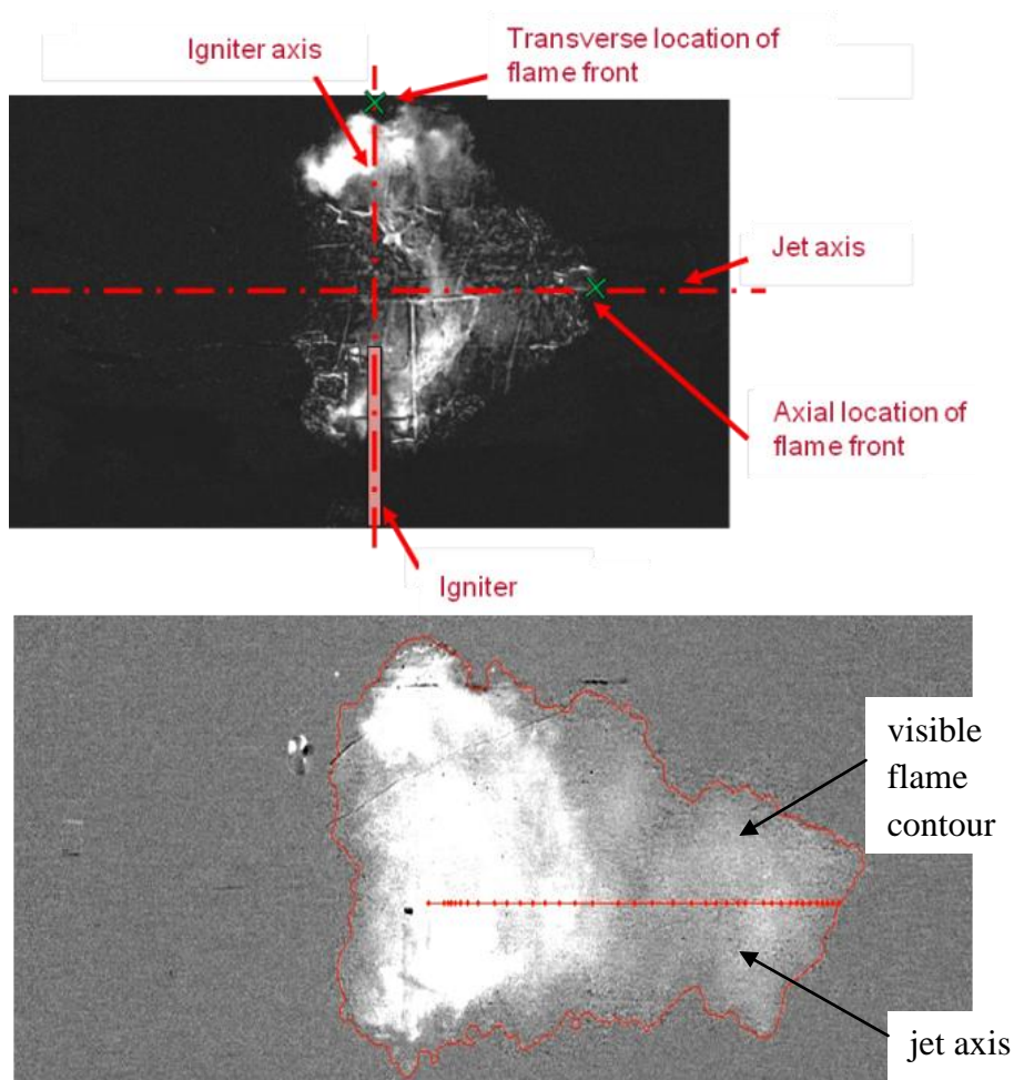
Figure 8 : flame front visualizations of one ignition test (side views), post-treated images
