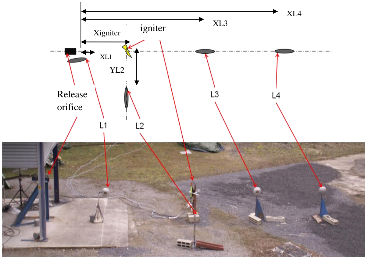
Figure 6: set-up of pressure sensors
