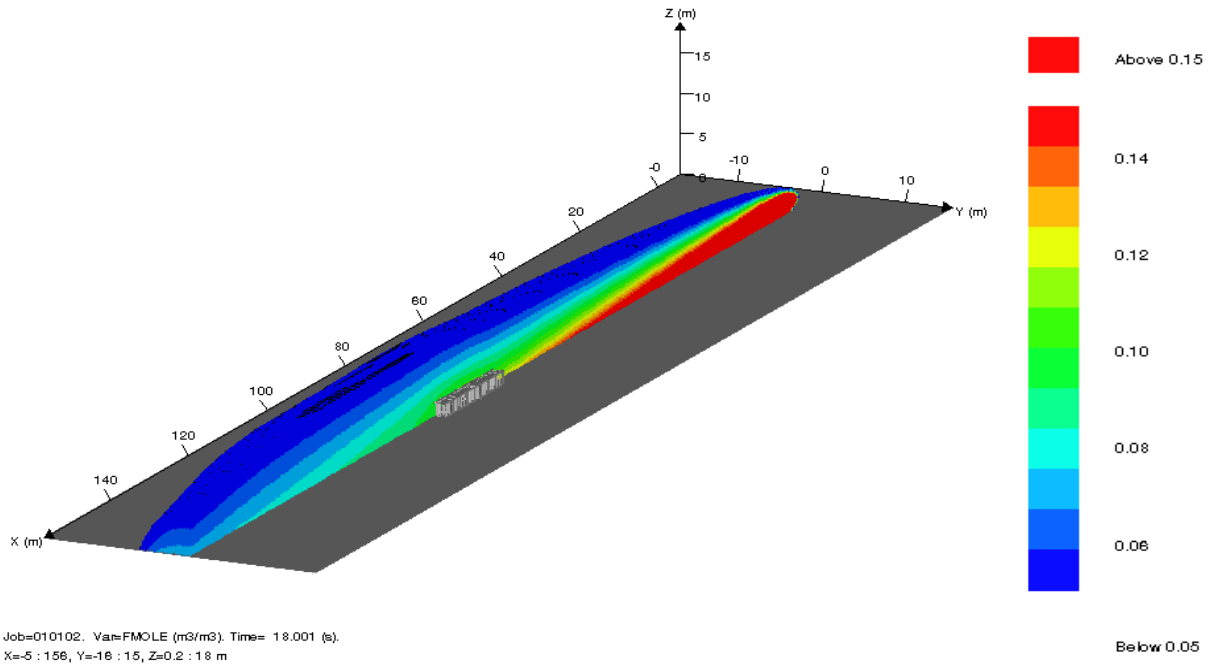
Figure 22 : 3D cut plane of the jet release covering the congested area (volume concentration)
