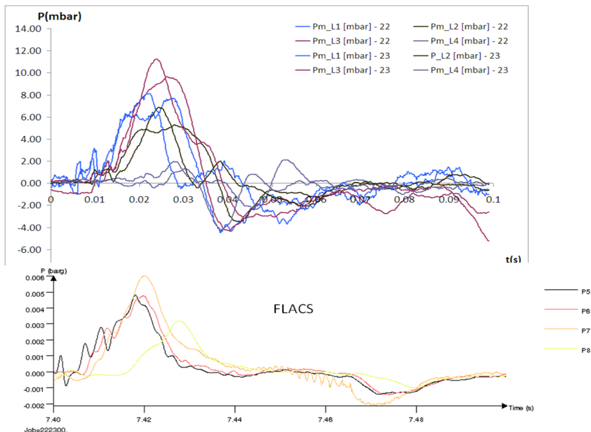
Figure 11 : pressure signal over time for different sensors positions, measured in the free gas jet ignition test (top) and calculated by FLACS (bottom)
