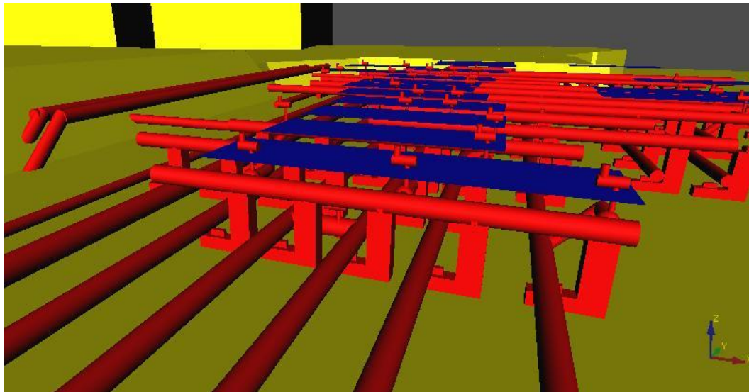
Figure 18 : example of large-size FLACS geometry
