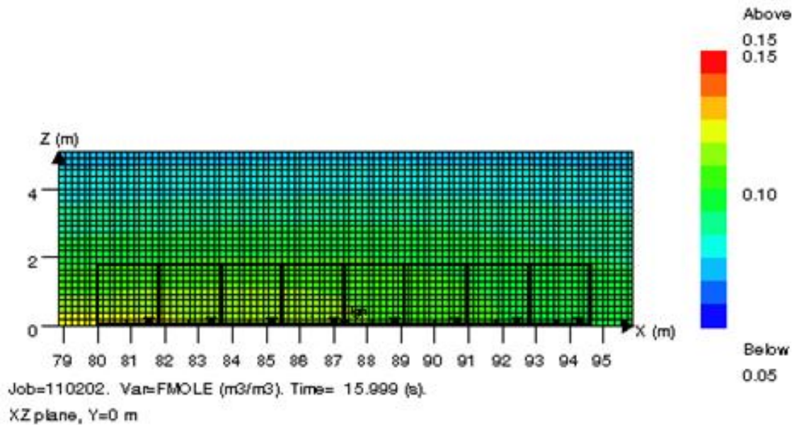
Figure 23 : 2D cut plane of the gas concentration along the jet axis
