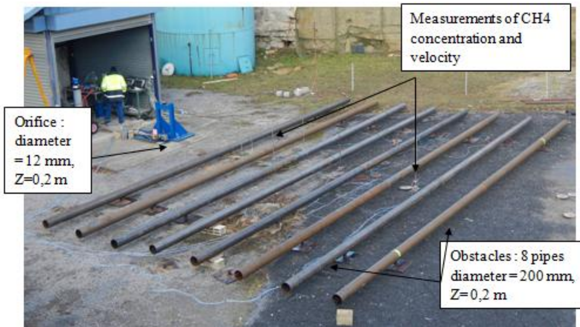
Figure 12 : test bench used by INERIS and GDF SUEZ for free methane jets
