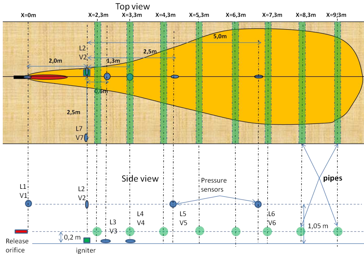
Figure 13 : locations of the release orifice, pipes, igniter and pressure sensors used by INERIS and GDF SUEZ for methane jets within a series of pipelines in parallel
