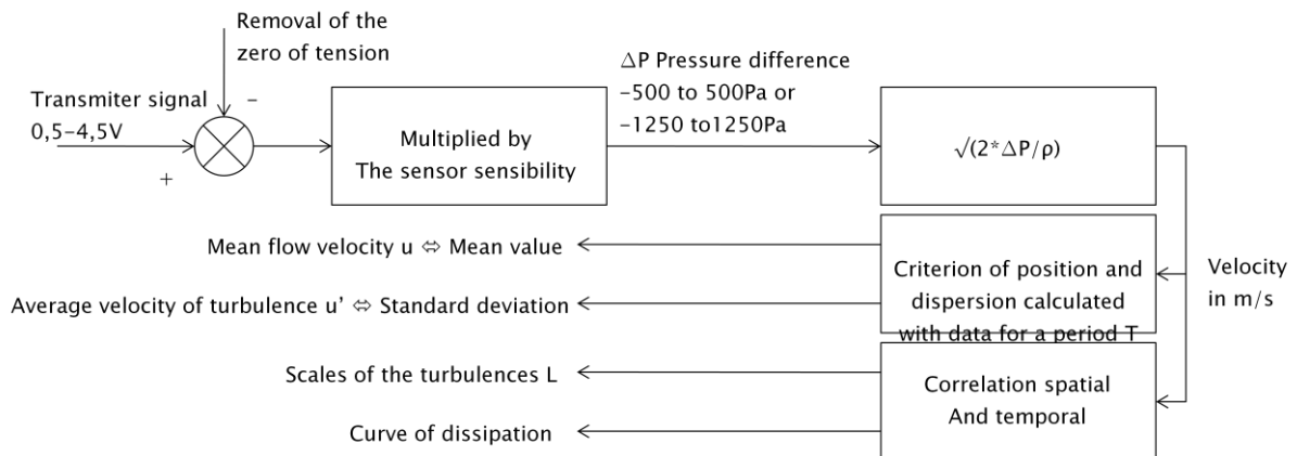
Figure 4: assessment of mean velocity, rms velocity and integral scale of turbulence from the signals of the differential pressure sensor mounted in the bidirectional Pitot probes
