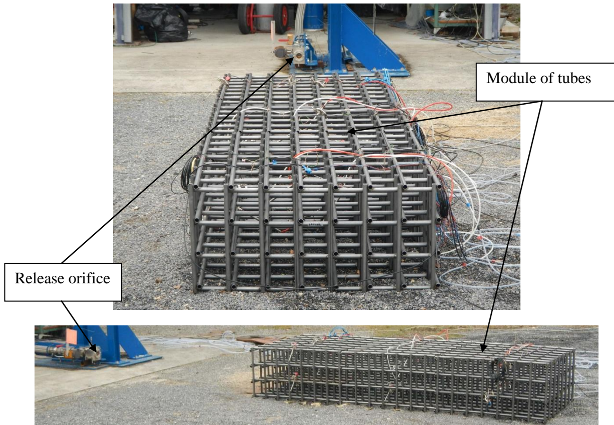
Figure 14 : 3D array of 20 mm diameter tubes used by GDF SUEZ and INERIS
