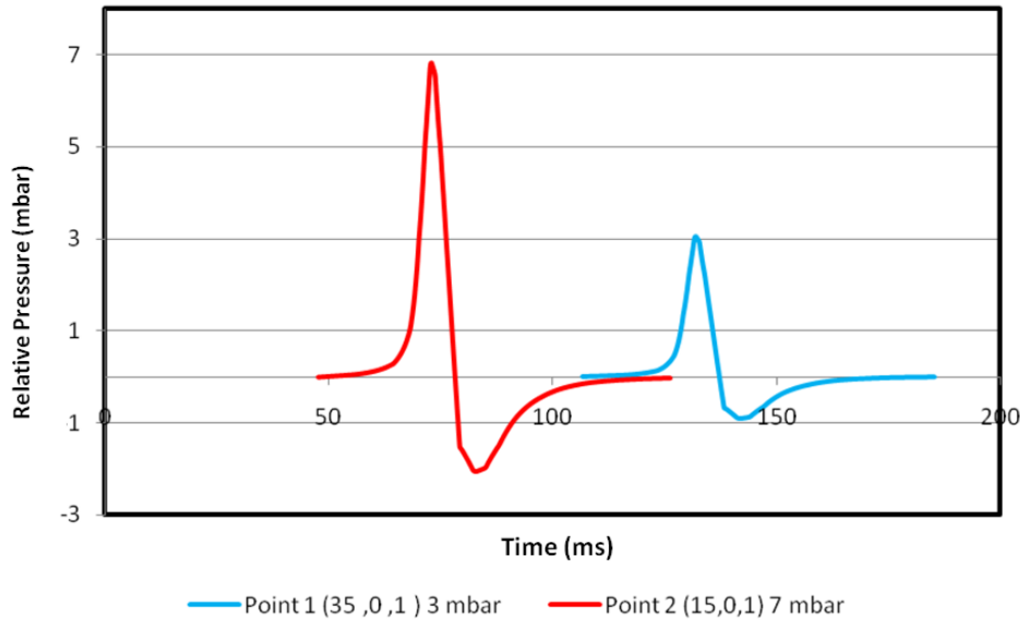
Figure 9 : overpressure signals for 1 ignition test of a free methane jet
