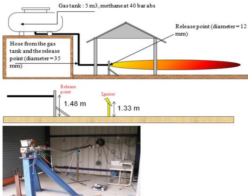
Figure 1 : test bench used by INERIS and GDF SUEZ for free methane jets
