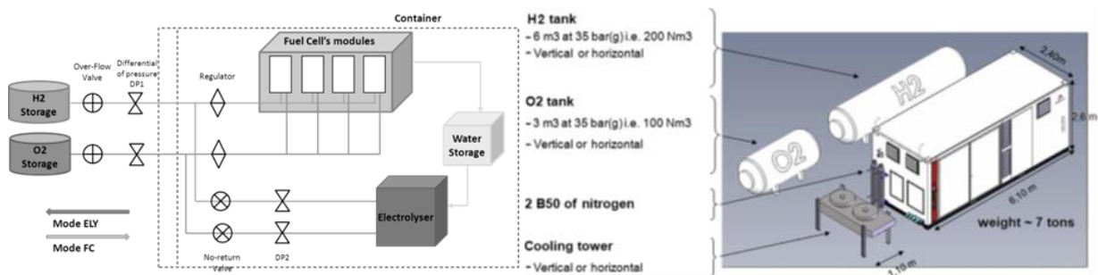
Figure 1. Illustration of the Greenergy Box TM [25]
