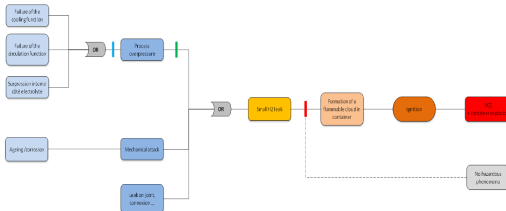
Figure 2. Bow-tie of “small leak of hydrogen in the container” scenario
