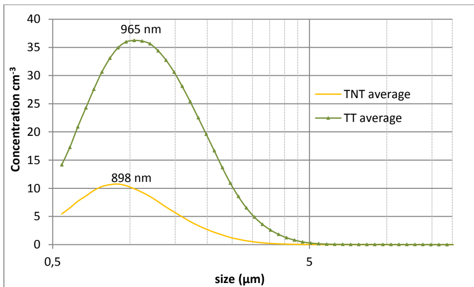
Figure 10: Size distributions (0.5 \mu\text{m} – 20 \mu\text{m} ) of particles released from treated (TT) and non-treated (TNT) tiles under abrasion, measured with APS. Each curve corresponds to an average of two tests.
