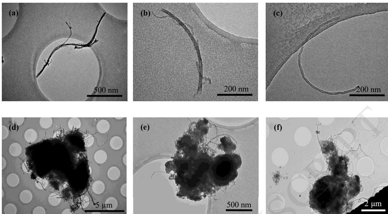
Figure 4: (a) - (d) Different forms of the sampled CNTs during extrusion process; (e) submicronic NOAA made of CNT and polymeric matrix (f) CNT bundle sampled during cleaning step of the PL6
