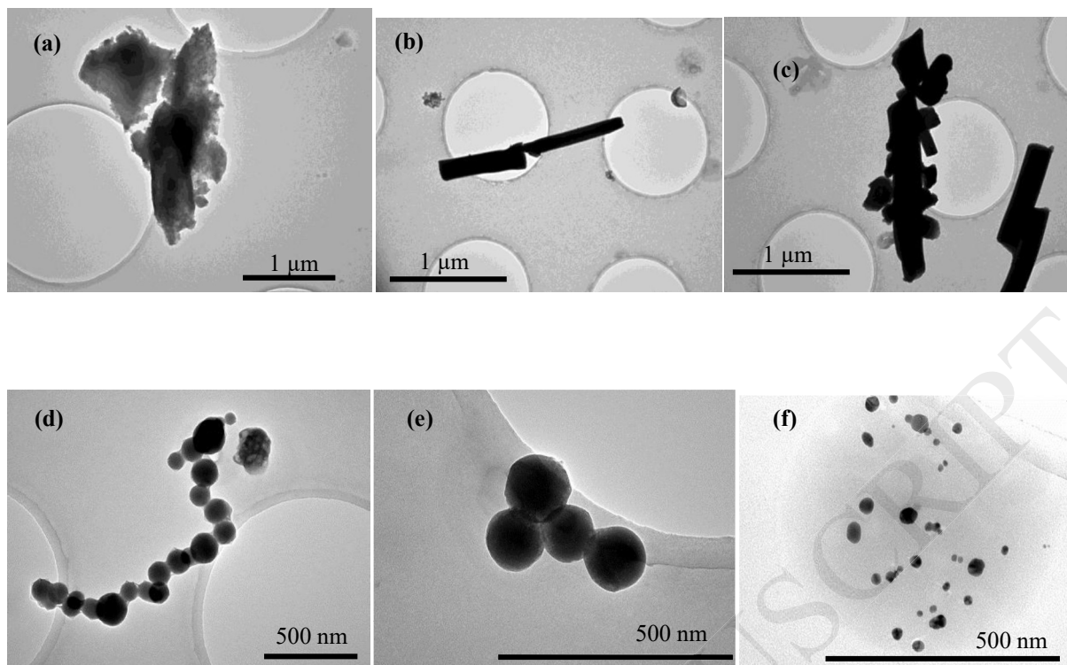
Figure 3: (a) TEM image of a particle containing Zr observed during opening of the oven and transport of the dried powder. (b) & (c) TEM image of the sampled aerosol particles during PL4 operation. (d) & (e) TEM images of the particles sampled during cleaning and filling steps; TiO 2 content: 1-2%; (f) Examples of NOAA of Ag and their clusters sampled during Ag based dispersion spray
