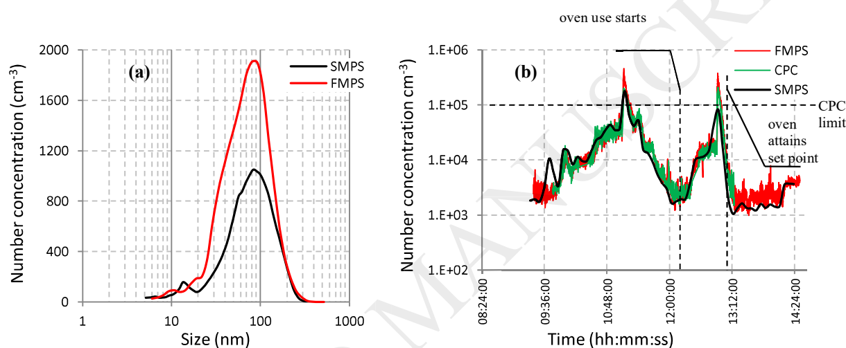
Figure 2: Comparison between (a) averaged particle size distributions of the emitted aerosol particles measured by SMPS and FMPS during the entire operation of PL1 (std. dev. for SMPS: 4 to 2094 cm -3 and for FMPS: 0.4 to 3615 cm -3 ); (b) total number concentrations measured by SMPS and FMPS with the number concentration measured by CPC during the entire operation of PL1
