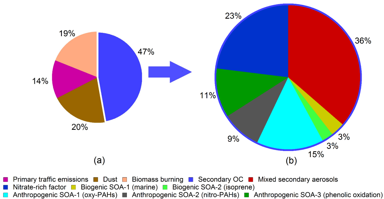
Figure 5. Average contributions of the identified sources to the total OC (POC + SOC) (left) and SOC (right) mass concentrations at Paris-SIRTA, France (March 2015).
