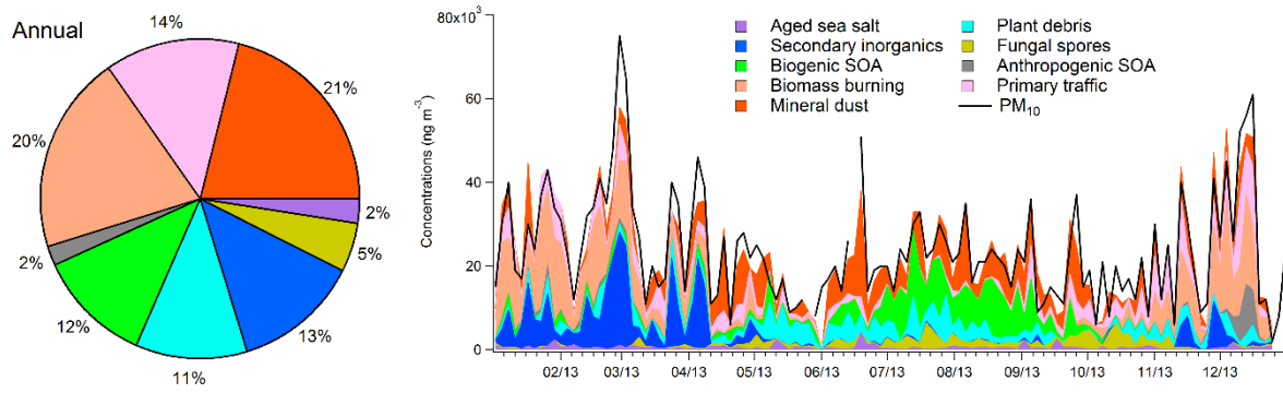
Figure 2. Annual average contributions (left) and temporal evolution (right) of the identified sources to PM 10 mass concentrations in Grenoble, Les Frènes (2013).
