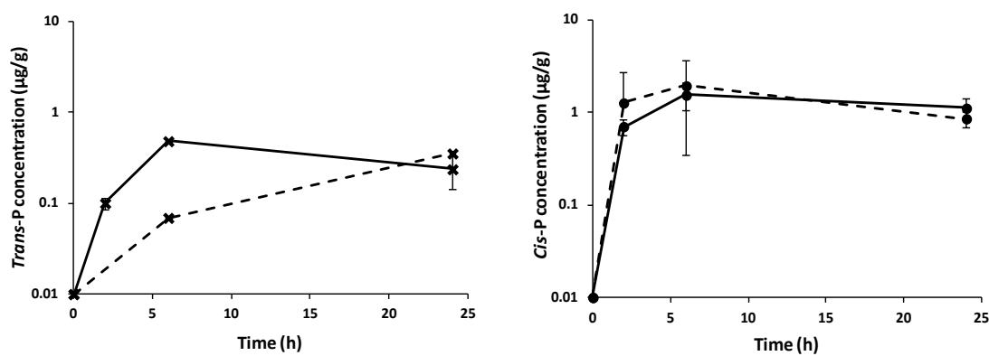
Figure 7: Cis -permethrin ( cis -P) and trans -permethrin ( trans -P) concentration vs. time profiles in fat after an oral administration of 5 mg/kg (dashed line) and 20 mg/kg (solid line) of cis - or trans -permethrin. Mean values \pm SD for n = 2 at each time-point.
