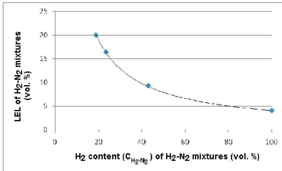
Fig. 2 : LEL variation of H 2 -N 2 mixtures versus their H 2 content C H 2 -N 2
