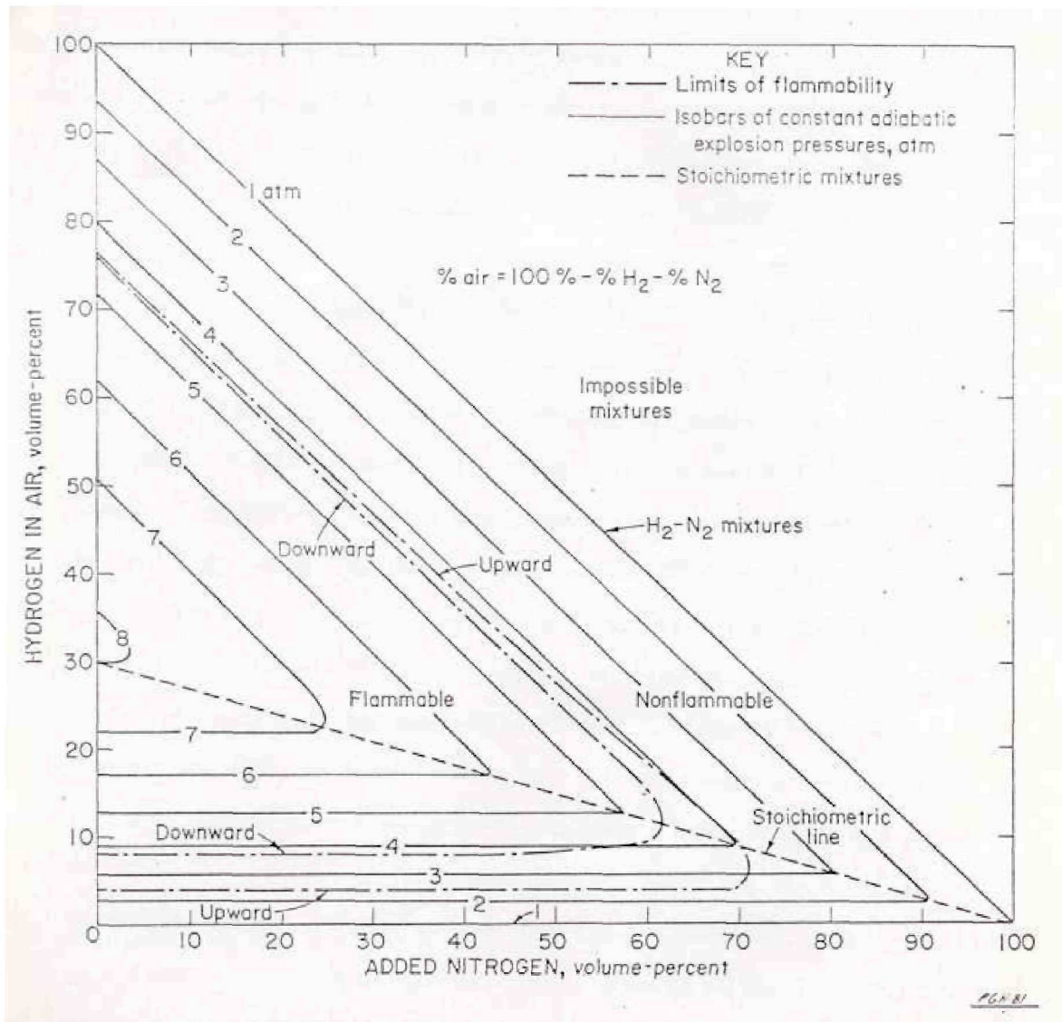
Fig. 1 : Ternary hydrogen-nitrogen-air diagram
