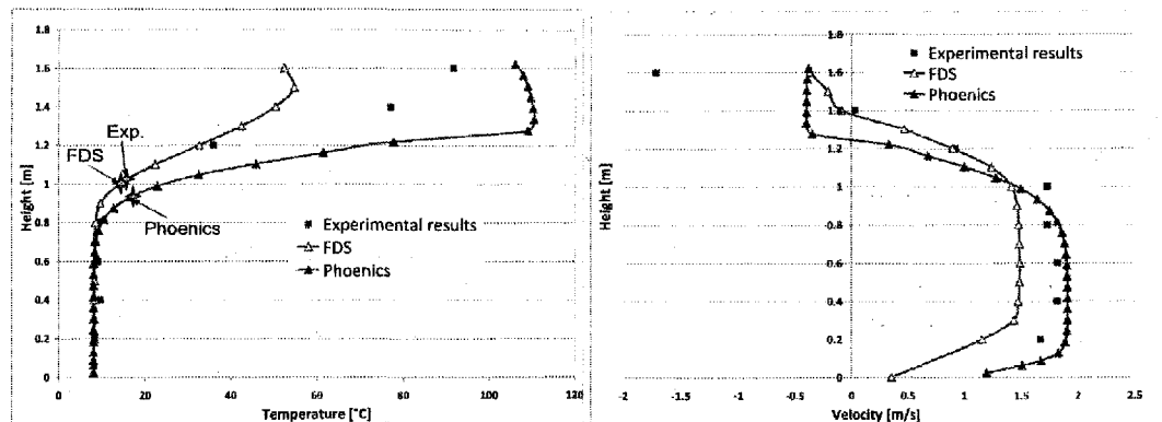
Figure 4: Temperature and velocity profiles comparison at 17 m upstream the fire.
