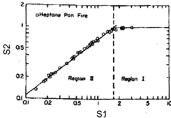
Figure 2: Evolution of the two stratification parameters, reproduced from (14).
