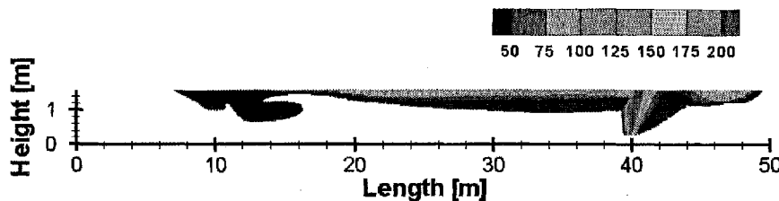
Figure 8: The backlayering layer front obtained with Phoenics
