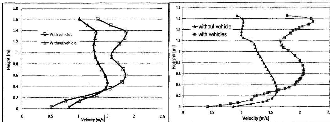
Figure 12: Evolution of the velocity profile in the centerline section, FDS on the left and Phoenix on the right.
