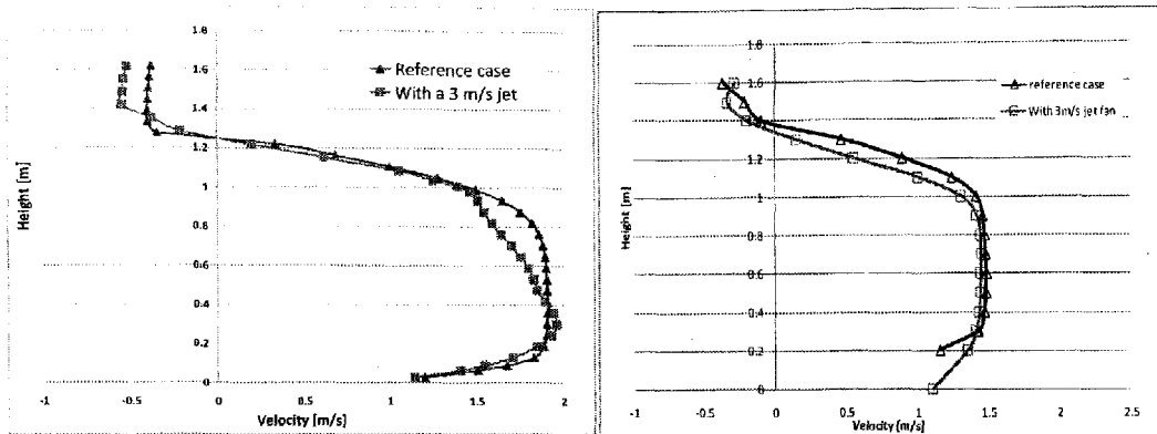
Figure 7: Velocity profile 17 m upstream the fire source obtained with Phoenics (left) and FDS (right).
