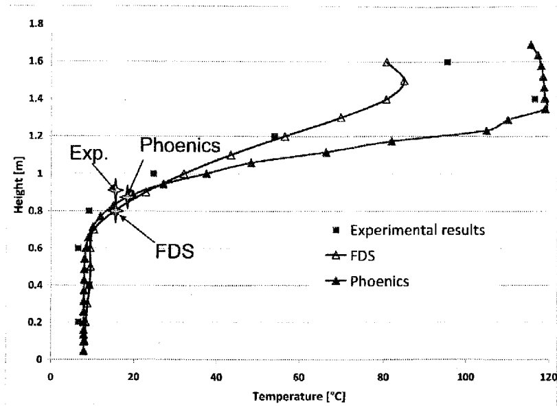
Figure 3: Temperature profile comparison at 10 m upstream the fire.
