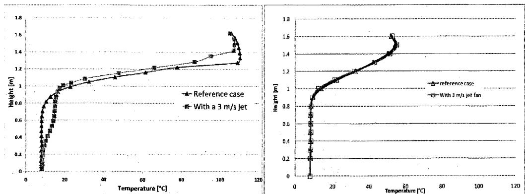
Figure 6: Vertical profile of temperature with and without jet fans at 17 m upstream of the fire obtained with Phoenix (left) and FDS (right).
