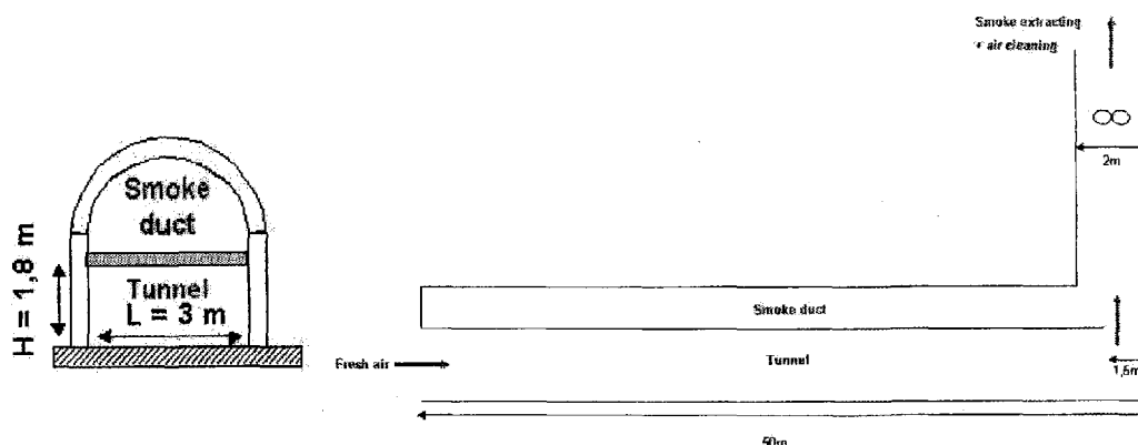
Figure 1: Scheme of the experimental set-up.
