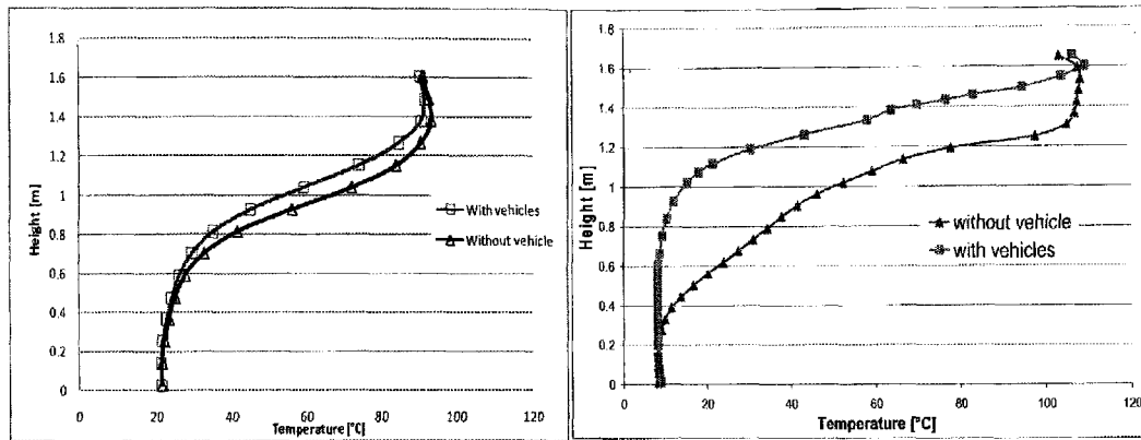
Figure 11: Vertical profile of temperature with and without vehicle obtained with FDS (left) and Phoenix (Right).
