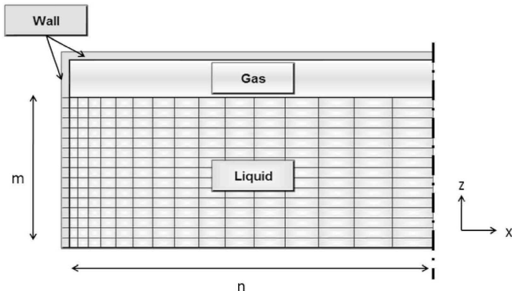
Figure 2. Axisymmetric mesh used
