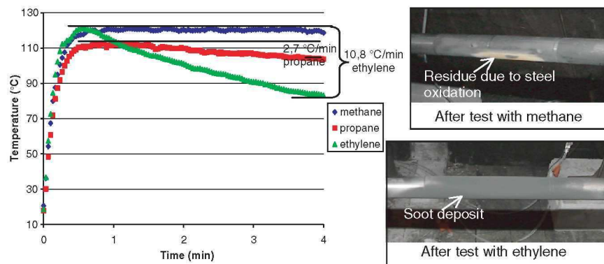
Figure 5. Evolution of the thermocouple directly impinged by jet fire and photos showing the consequences of jet fire
