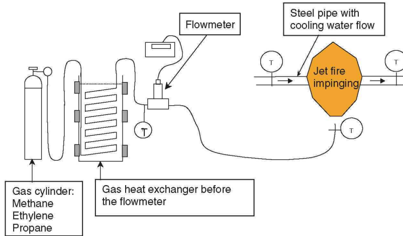
Figure 1. Sketch of the experimental apparatus
