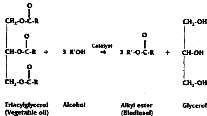
Figure 4: the chemical reaction of transesterification
