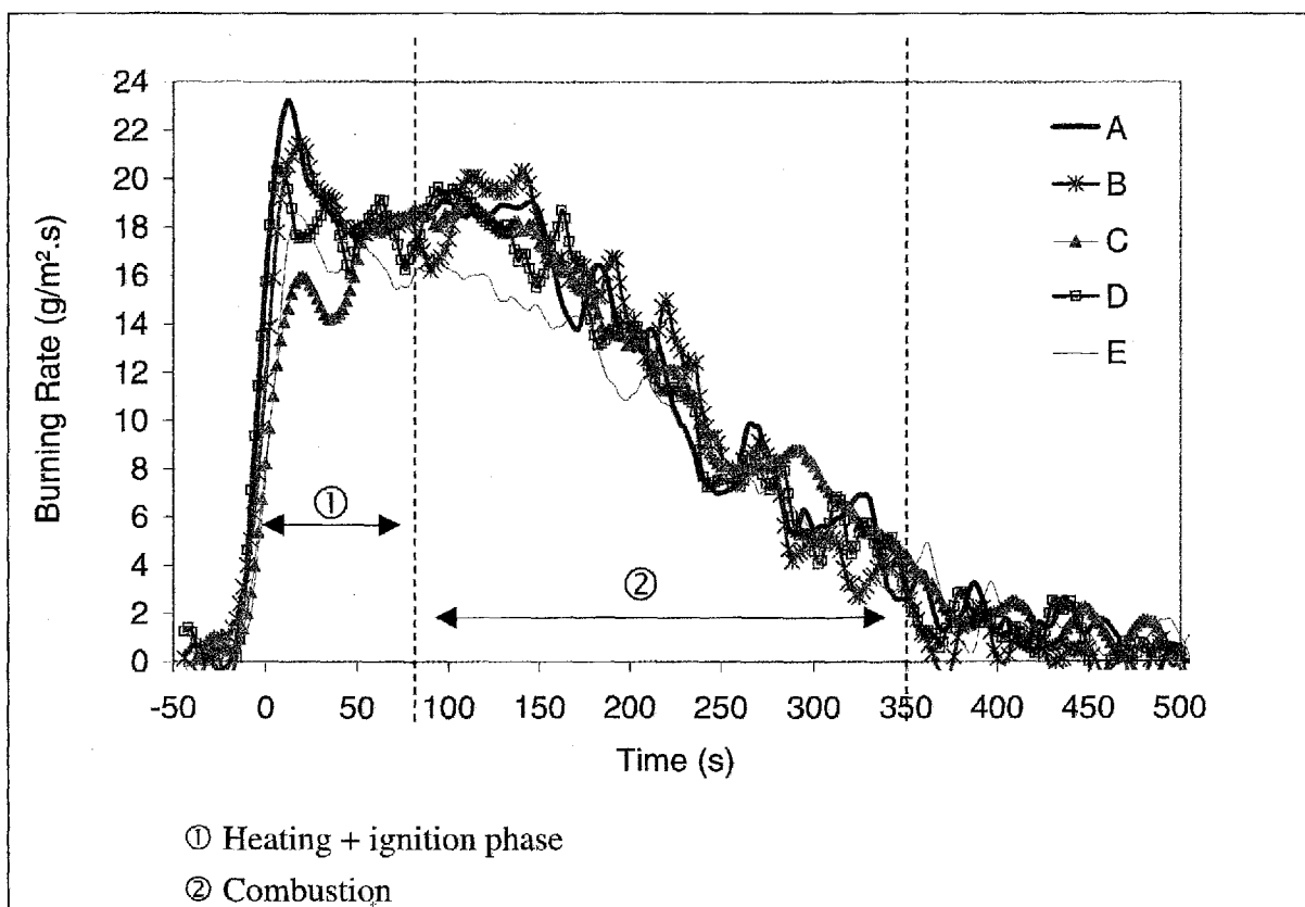
Fig. 4. Burning rate versus time at 50 kW/m 2 for (A) PVC, (B) PVC + 0.2% Sb 2 O 3 , (C) PVC + 3% Sb 2 O 3 , (D) PVC + 0.2% ATH and (E) PVC + 3% ATH
