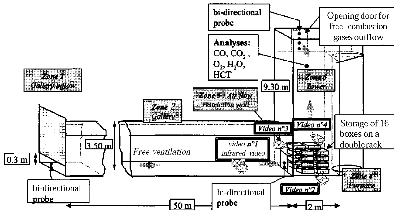
Figure 1 : Use of the fire gallery for the campaign
