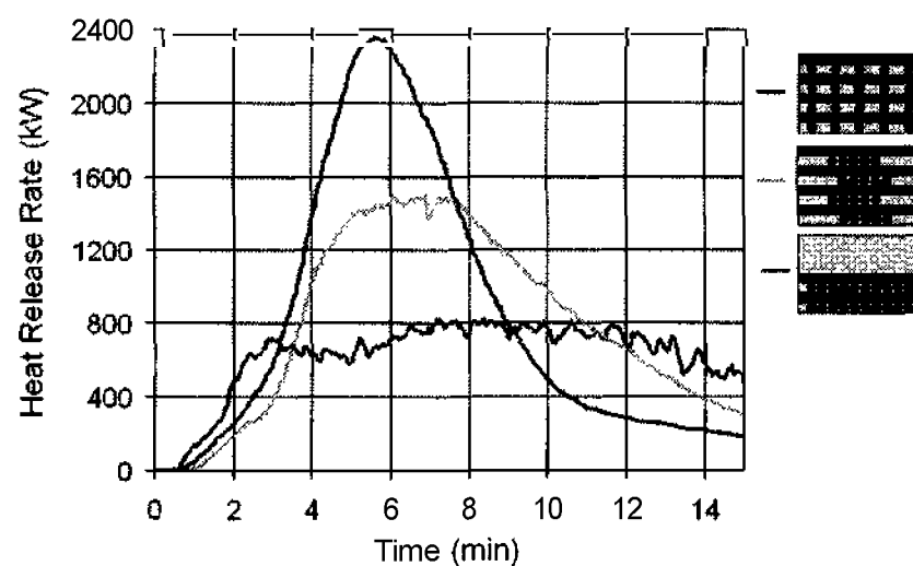
Figure 8: Influence of sticks arrangement on HRR
