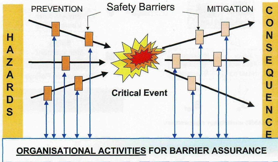
Figure 2. Bow-tie approach for scenario identification
