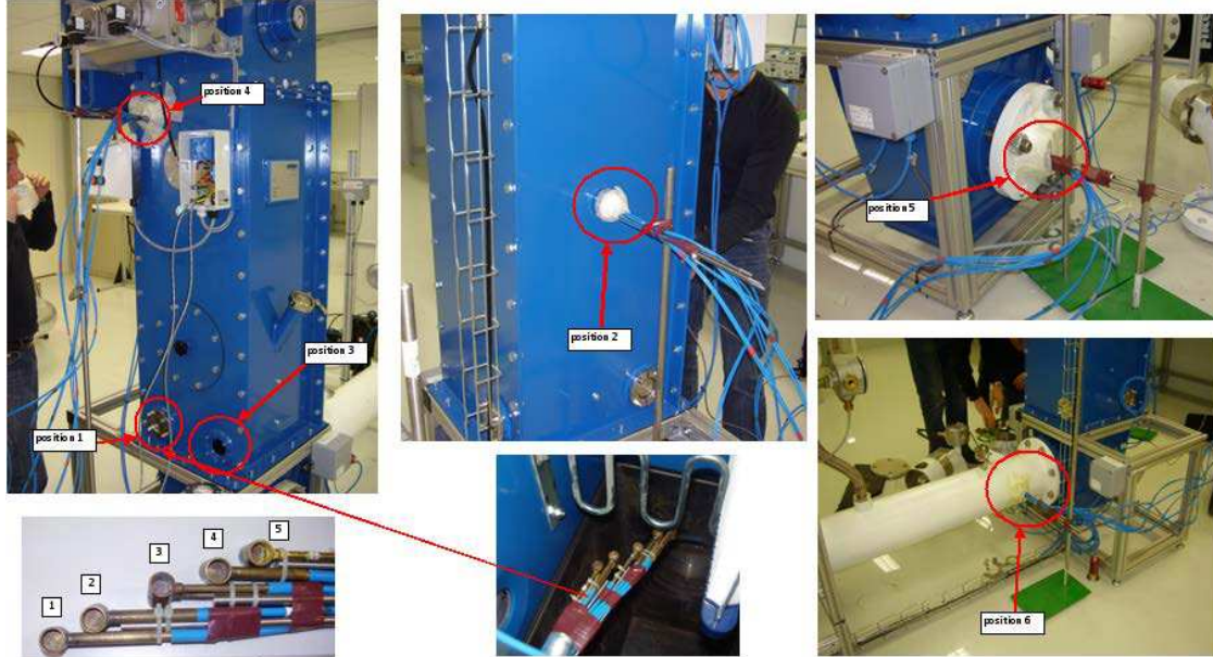
Figure 9: locations of the measuring points in the filter (location 6 is on the inlet pipe, 1&3 below the sleeves, 2 between the sleeves, 4 top between wall and sleeves)
