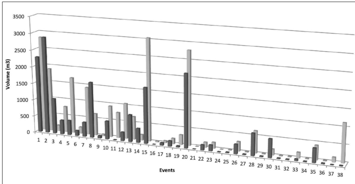
Figure 8. The high likelihood region of the location pdf, V_{pdf} , for the real events versus the number of events is presented. In light grey the values obtained with a 3D velocity model with cavity, in dark grey without cavity
