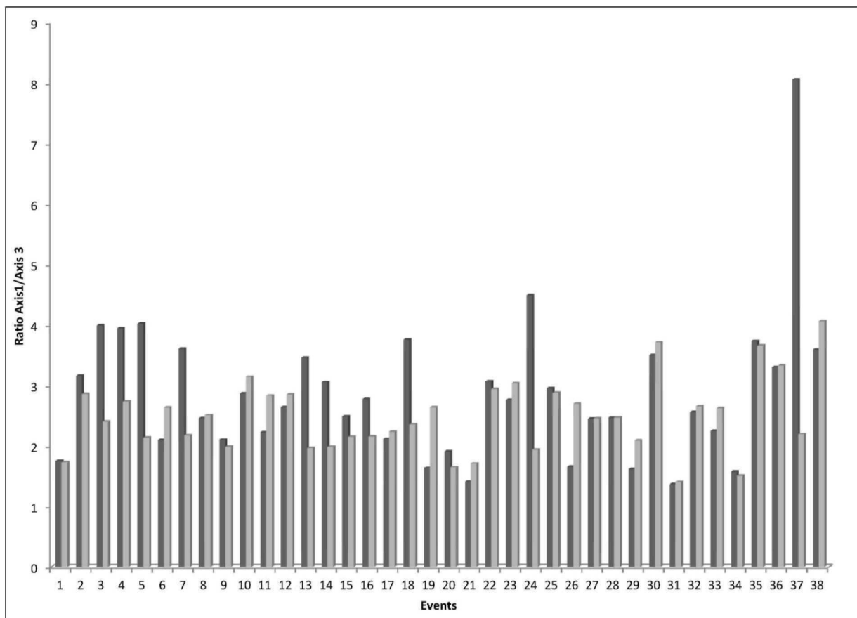
Figure 7. The ratio between the maximum axis (Axes 1) and minimum axis (Axes 3) of a 68% confidence error ellipsoid versus the number of events is presented. In light grey the values obtained with a 3D velocity model with cavity, in dark grey without cavity
