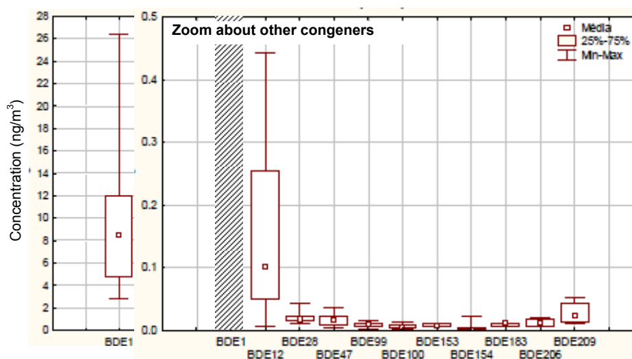
Figure 4. Box plot of PBDEs congeners concentrations (ng/m 3 ) for active air samplings
