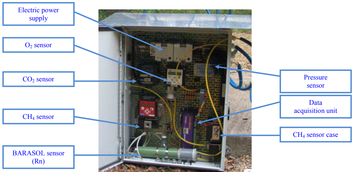
Figure 4: Monitoring station.
