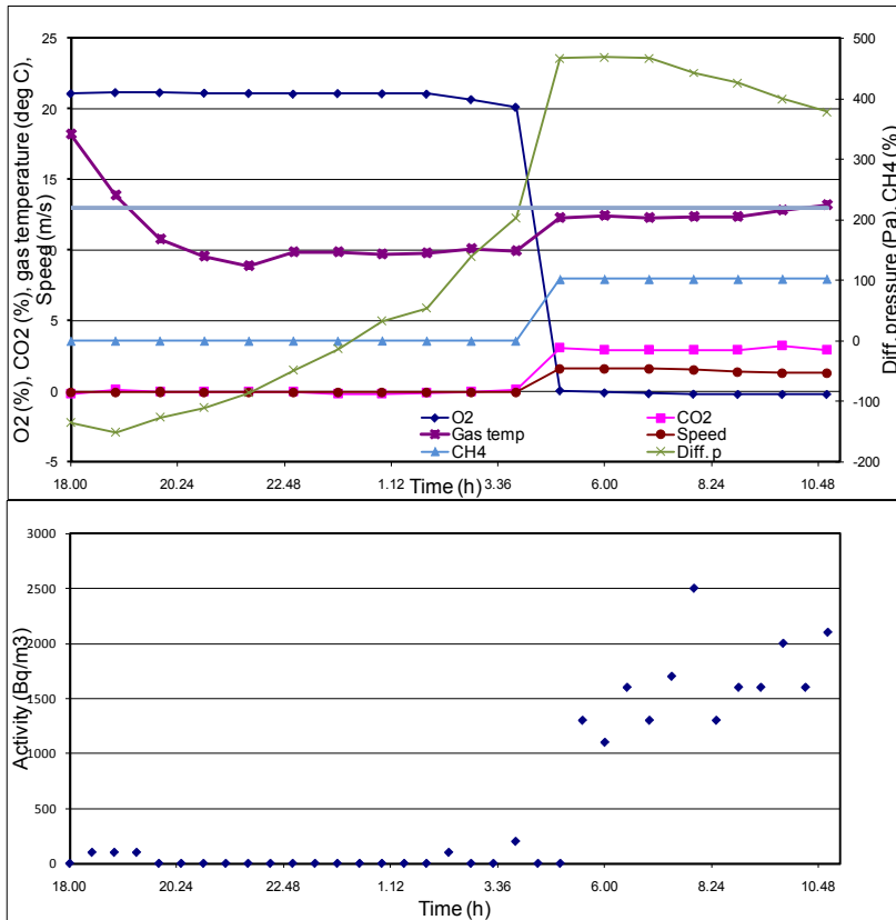
Figure 5: Variations in gas and radon content at Barrois shaft from 09/10/2007 to 10/10/2007.
