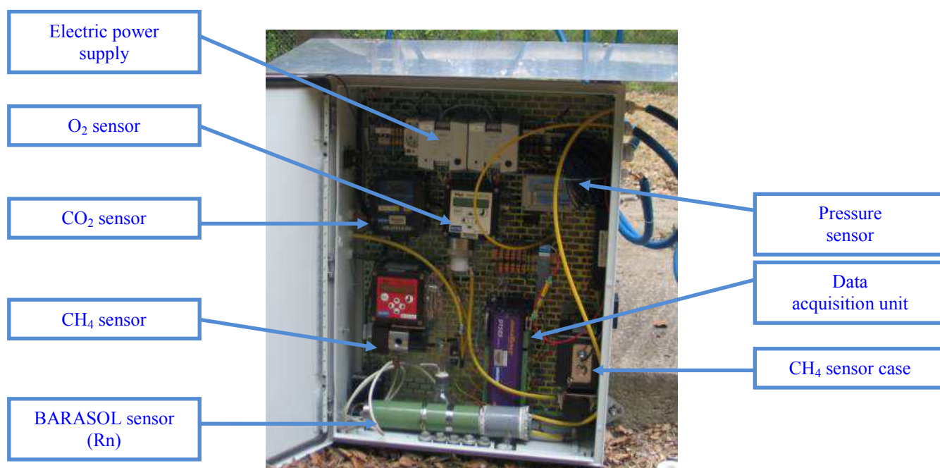
Figure 4: Monitoring station.
