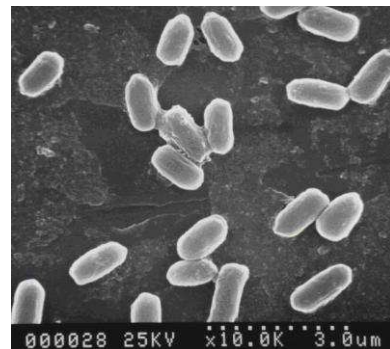
Figure 2. Spores of B. atrophaeus (MEB)
