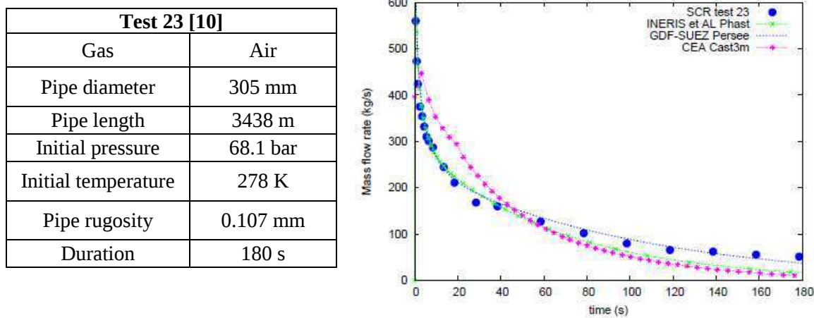
Figure 1: Comparison between all pipeline decompression models
