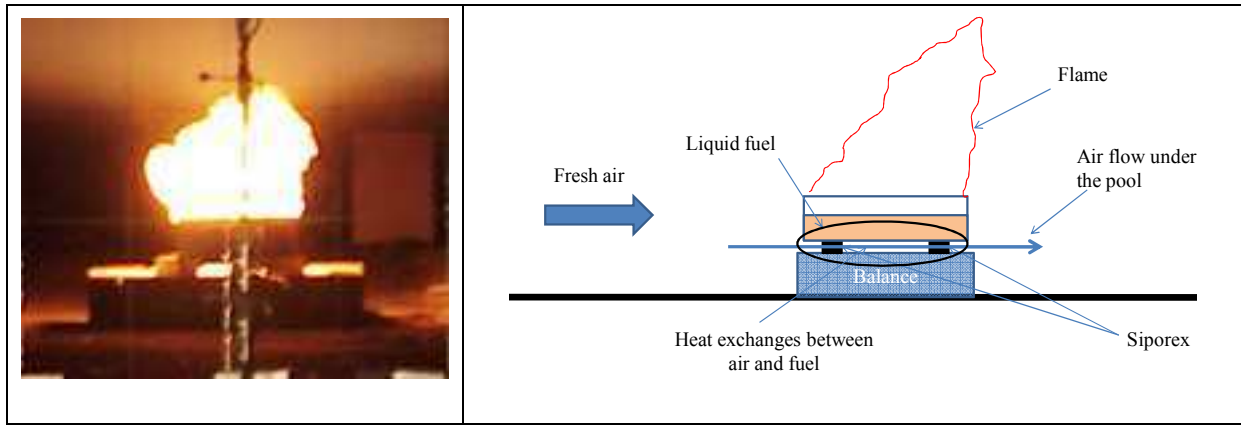
Fig. 7 Photography (left) and scheme (right) of the experimental set-up for fire
