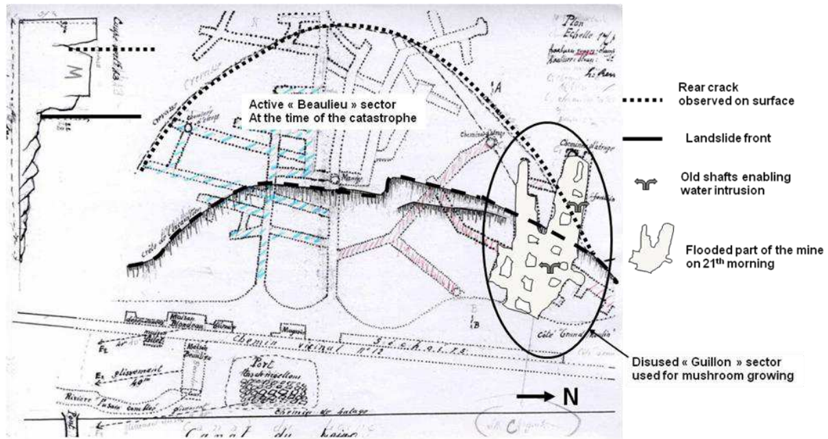
Figure 6: Schematic view of the collapse and associated landslide of the Lorry hillside on January 21 st , 1910.
