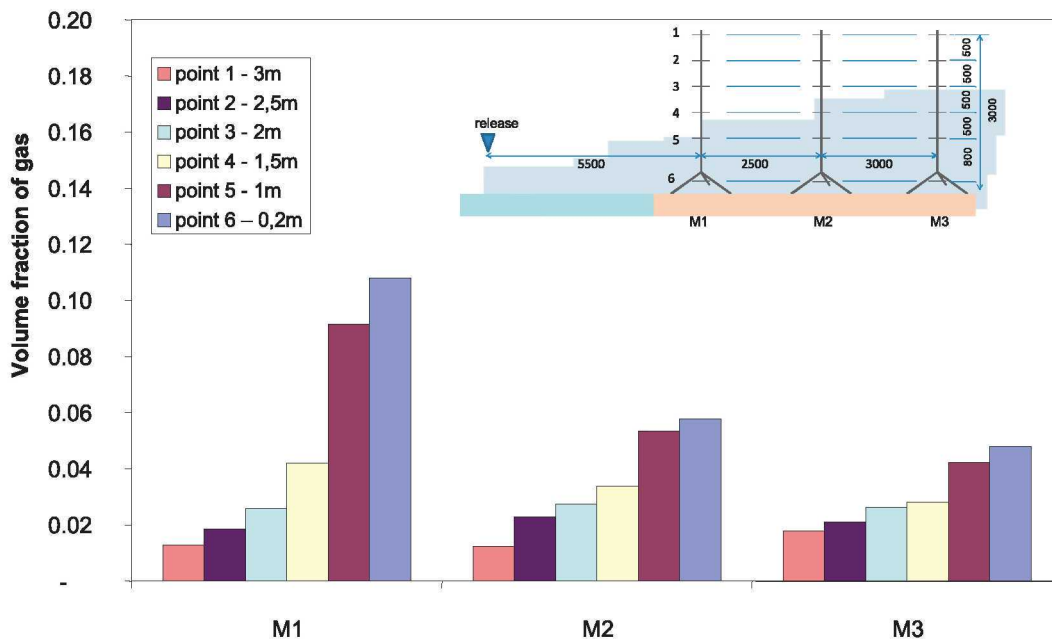
Figure 7: Calculated mean N 2 concentrations at the three atmospheric masts for trial No.7.
