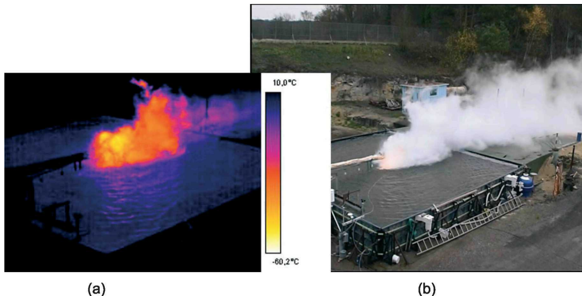
Figure 4: Images extracted from (a) thermal and (b) traditional videos of trial No.7
