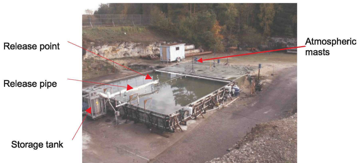
Figure 1: Experimental device
