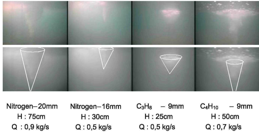
Figure 5: Underwater mixing cones for different test cases. H: cone depth – Images extracted from trials No.7, 9, 13 and 16 respectively.
