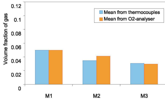
Figure 6: Comparison of the averages of nitrogen concentrations measured and deduced from formulation (1) for trial No.7
