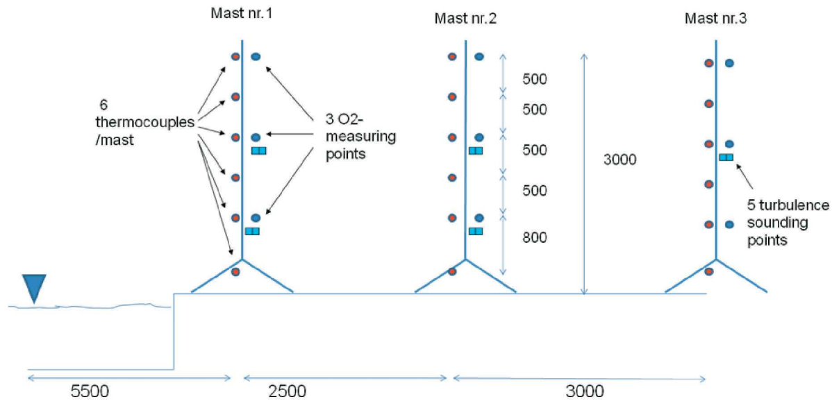
Figure 3: Atmospheric measurement equipment – Nitrogen is measured by means of a sampling device connected to an O 2 -analyser
