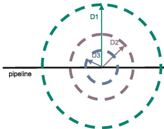
Figure 2: Effect distances for one phenomenon (ie jet fire after a small leak)
