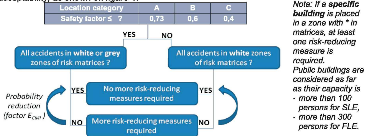
Figure 4: Risk control process for existing exposed population
