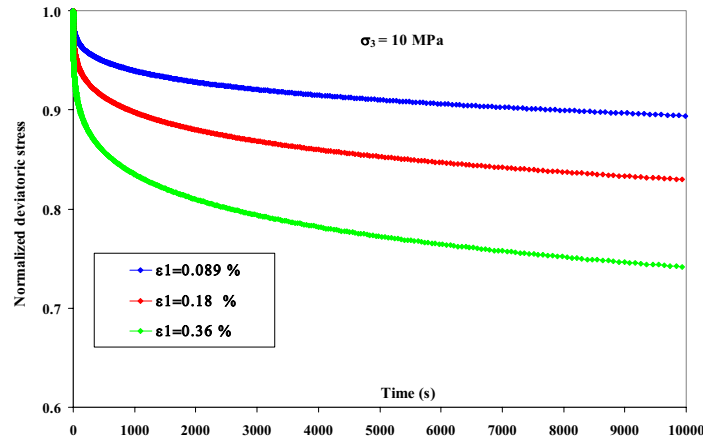
Fig. 6. Simulation of relaxation test per stage ( \sigma_3 = 10 MPa) at three levels of deviatoric stress ( q = \sigma_3 - \sigma_1 ): q = 5 MPa ( \epsilon_1 = 0.089\% ), q = 10 MPa ( \epsilon_1 = 0.18\% ) et q = 25 MPa ( \epsilon_1 = 0.36\% )
