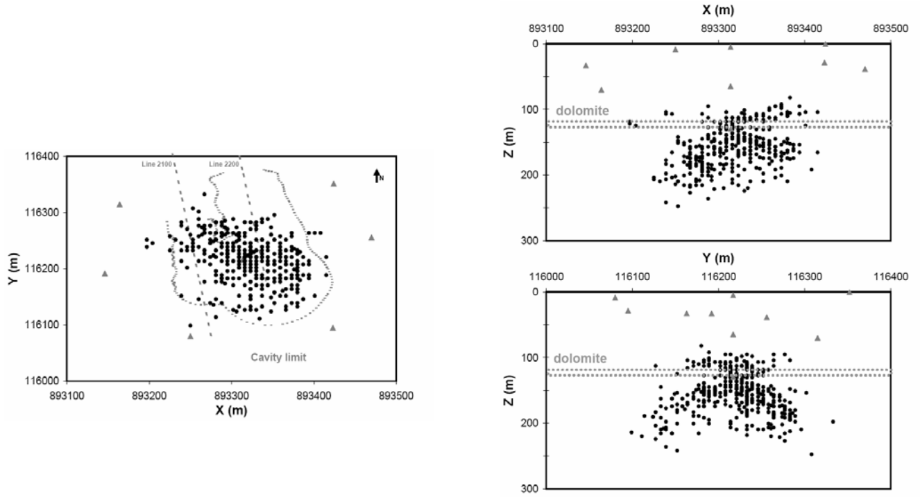
Figure 5: Positions of the microseismic events (black symbols) and of the microseismic sensors (grey triangles) along cross sections XY, XZ and YZ for the episode on 12 March 2008.
