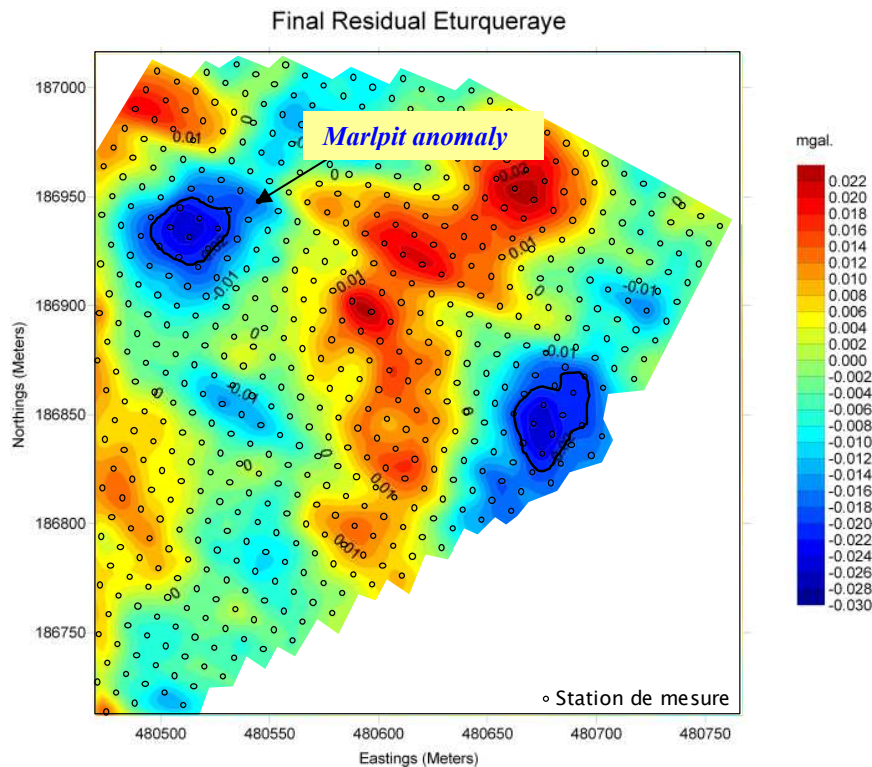
Figure 10. Gravity residual anomalies obtained for the marlpit site Etruquay
