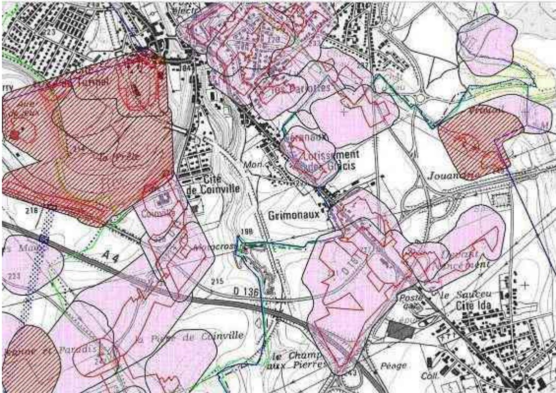
Figure 4 Example of a hazard map in the Lorraine iron ore field (North-East of France)
