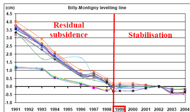
Figure 3: Example of the Billy-Montigny levelling line. The stabilisation of the residual subsidence is clearly observed after 1999.
