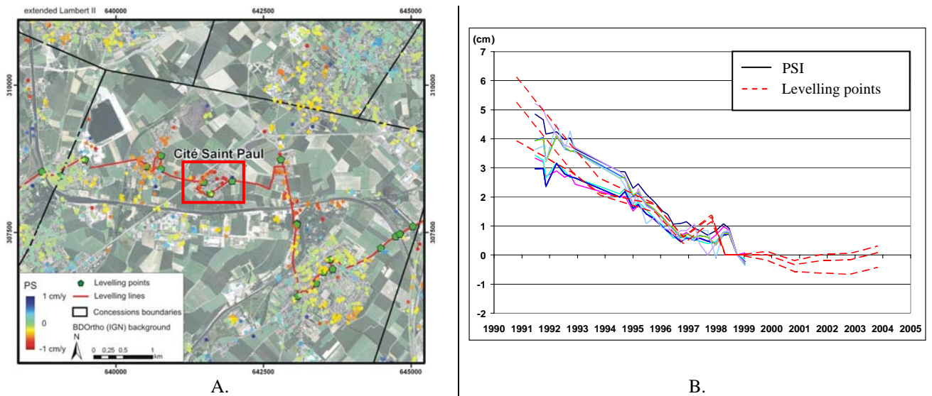
Figure 6: Comparison between PS displacements and levelling monitoring in the "Cité Saint Paul" area for PS closer than 150m of the levelling point. A.: Localisation of the "Cité Saint Paul" area and considered data (red square). B.: Comparison of PS and levelling results where dashed lines represent the levelling points and continued lines, the PS.
