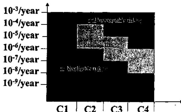
Figure 3: Risk matrix used for ranking the dangerous phenomena and selecting the Reference Accident scenarios for the risk severity mapping
