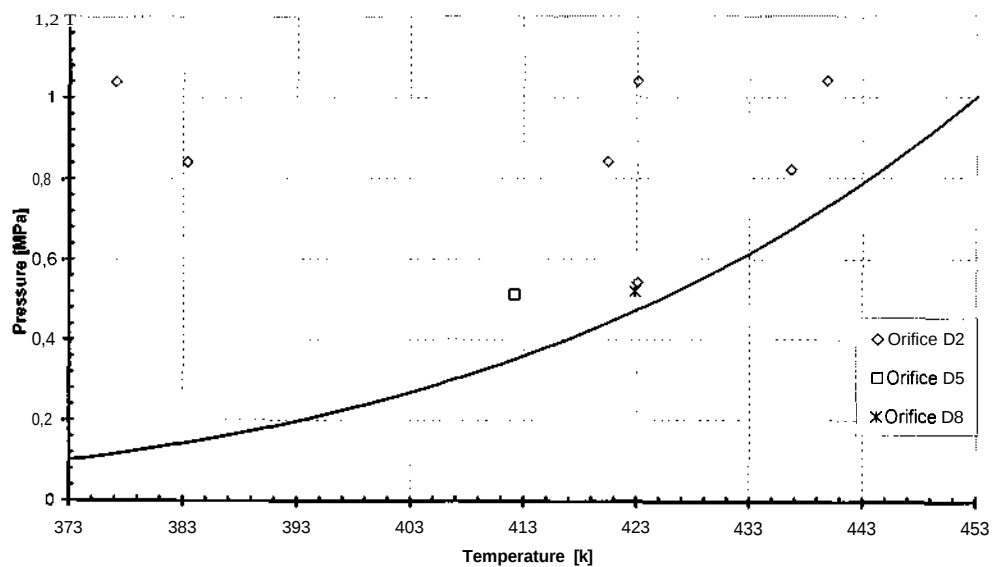
fig. 8.: Experimental reservoir conditions. Waterjets from orifices.
