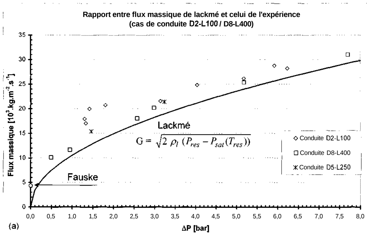
Fig 11. : mass velocity versus (P_{res} - P_{sat}(T_{res})) (pipes)
