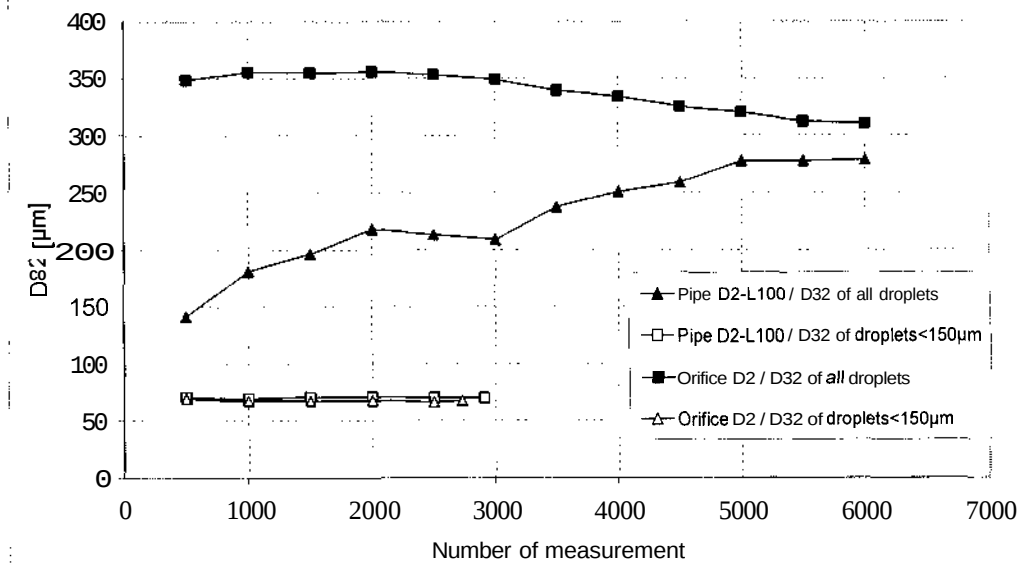
Fig 7.: d_{32} measurement accuracy versus droplet number (small droplets ; whole population).
