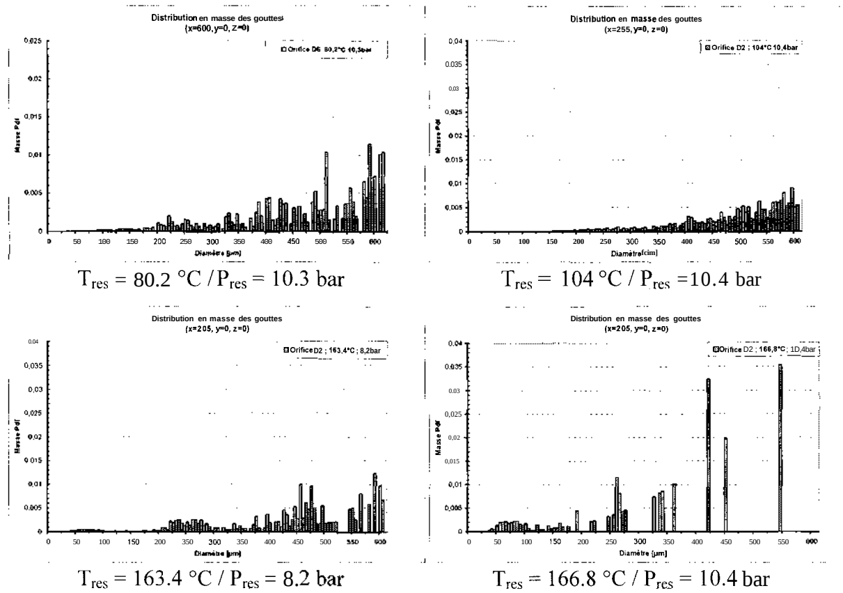
Fig. 20. : mass size distribution at différent reservoir conditions (200 mm down-stream from D2 orifice)
