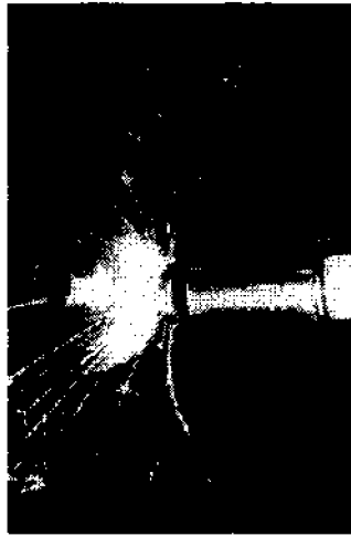
Figure 1 : example of a « spark shower » from Ritter 1984
