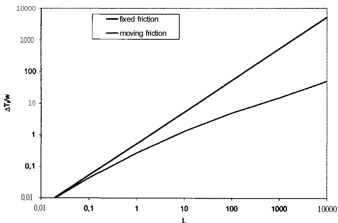
Figure 2 : Temperature difference ( \Delta T ) of the hot spot with the mean body temperature as function of L = V \cdot R / 2 . \alpha , w = \pi \cdot q / A . p , c . V , \alpha is the mean thermal diffusivity of the bodies, c the specific heat, and R the typical size (radius) of the heated zone.
