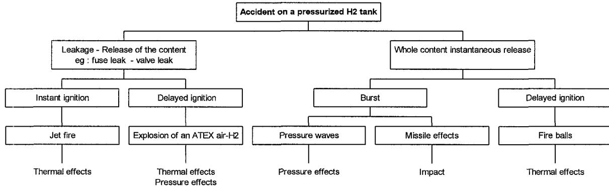
Figure 3: Tank accidental situations
