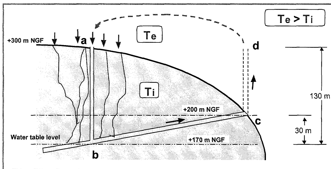
Figure 3. Schematic diagram of the natural thermal draught during the summer period (Moyeuivre-Grande reservoir case)
