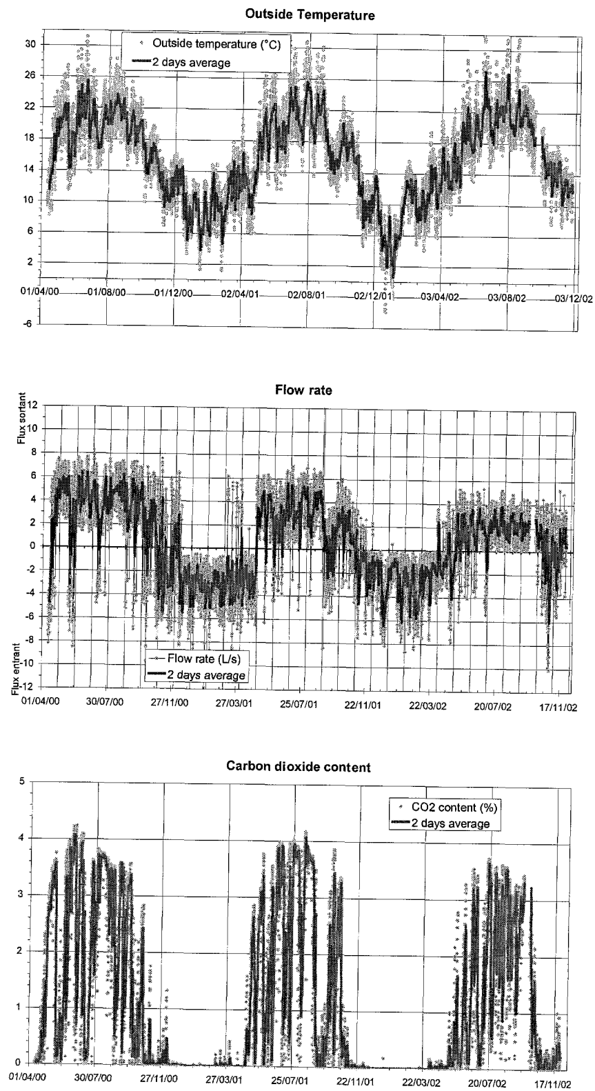
Figure 2. Outside temperature, air flow rate and CO 2 content evolutions observed in a gallery connected to the Moyeuve-Grande reservoir.
