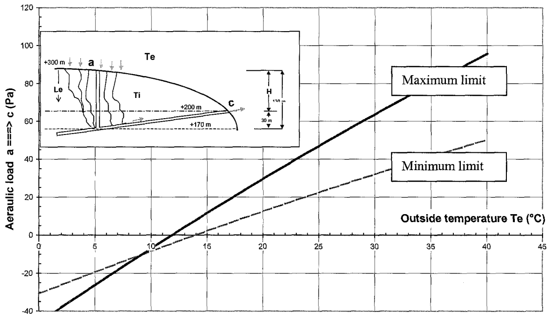
Figure 5. Estimation of the aeraulic load thanks to the hydrostatic method (with non modified dry air).
