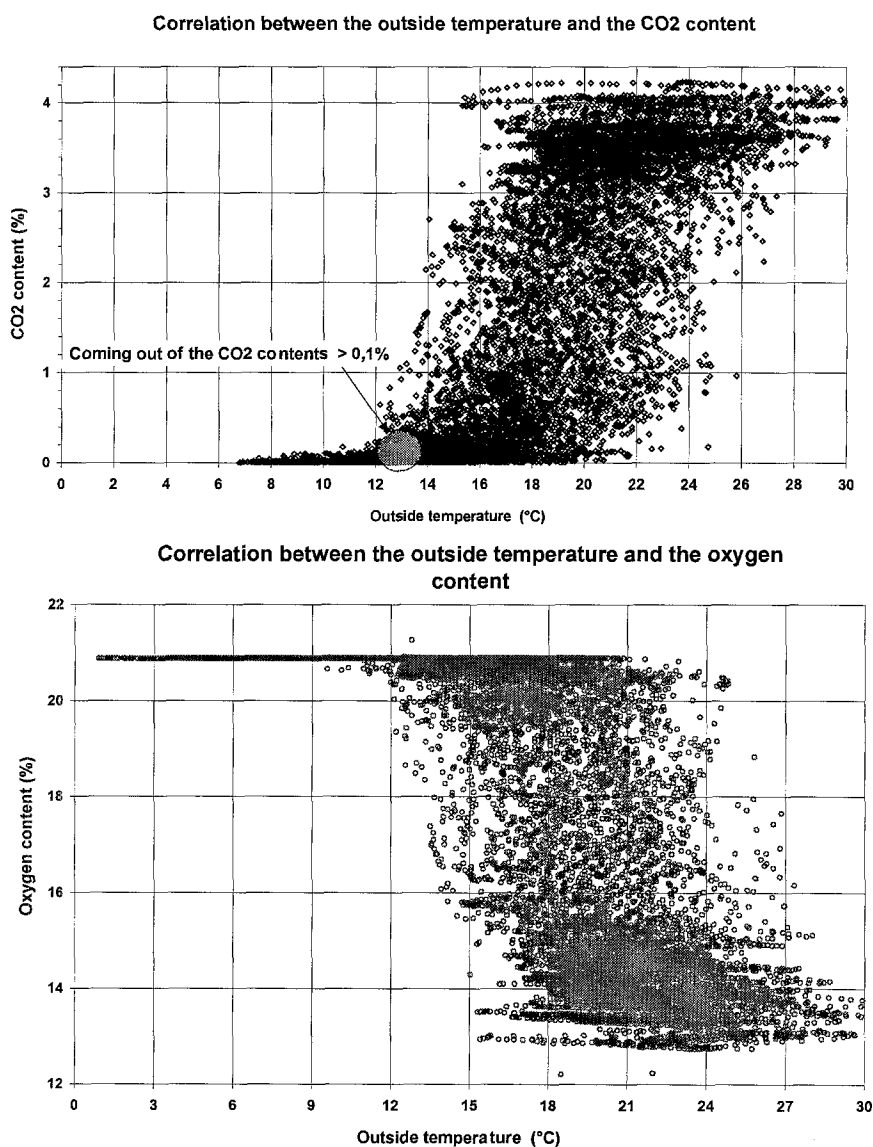
Figure 4. Correlation between the outside temperature and the O 2 and CO 2 contents observed in an opening of the Moyeuivre-Grande reservoir
