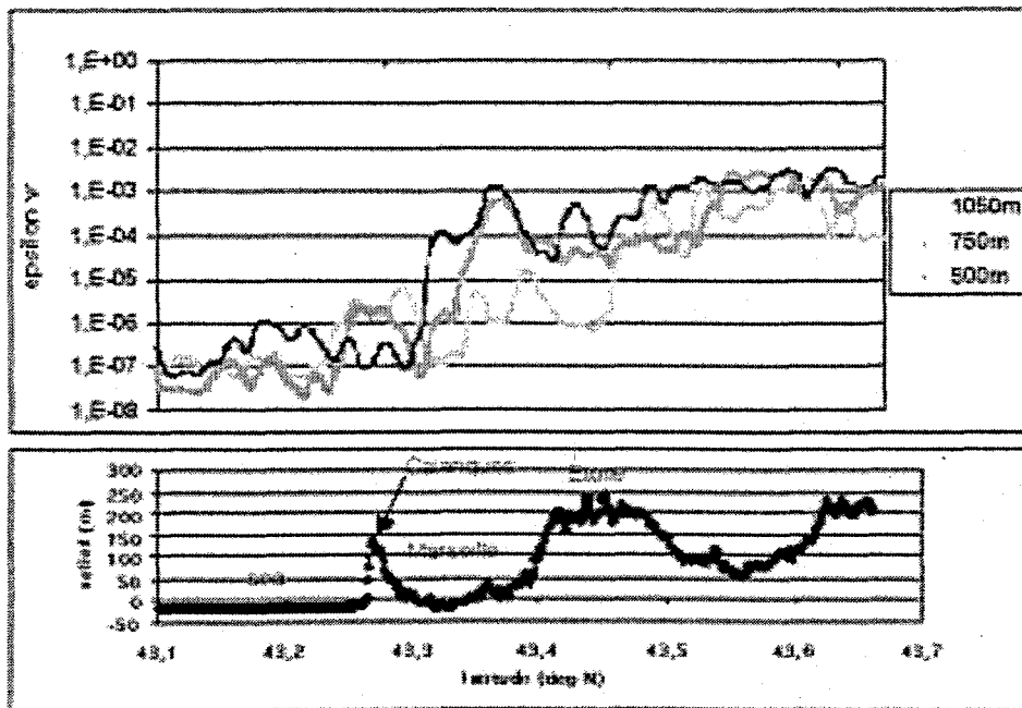
Figure 3. Dissipation rate of turbulent kinetic energy ( m^2s^{-3} ) measured with the Merlin IV (MeteoFrance) along the south-north legs at levels 1050, 750 and 500 m. The overflow relief is also represented with the sea on the left (south). The duration of the flight over the town, between the Calanques ridge to the south and the Etoile massif to the north, is 3 minutes. The energy spectrum high frequency tail is a relevant indicator of turbulence intensity in such inhomogeneous conditions.
