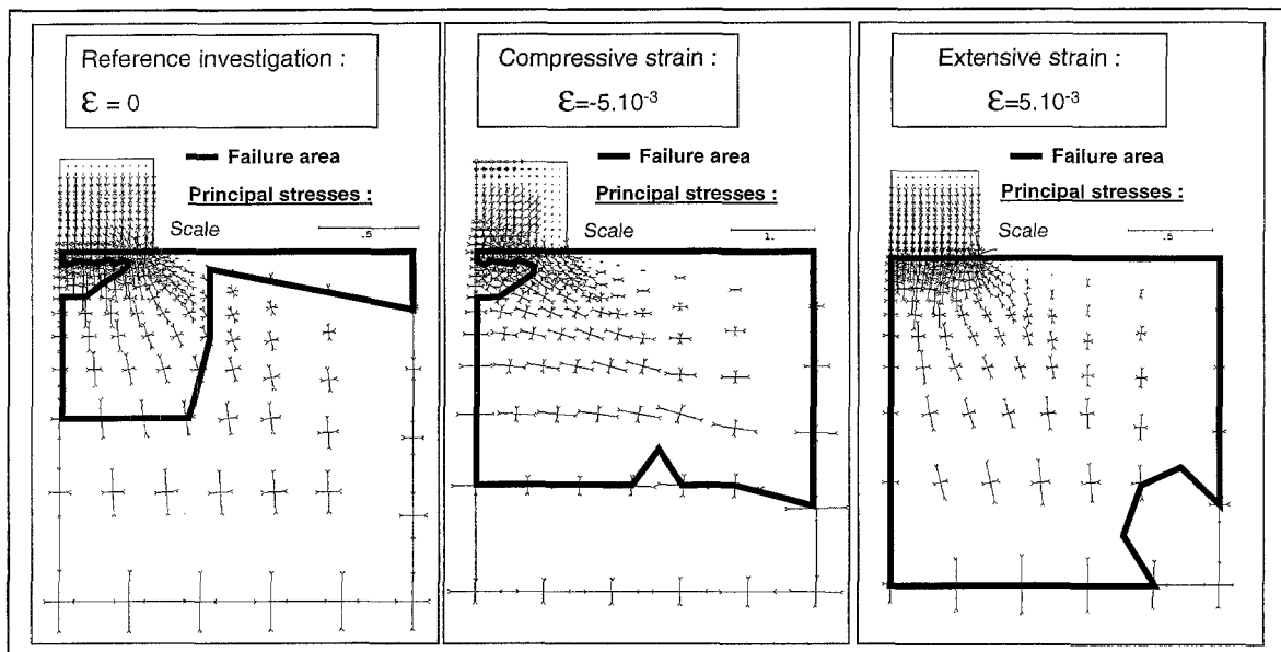
Figure 6: Stress fields and failure areas in a strain area ( \pm 5 \cdot 10^{-3} )
