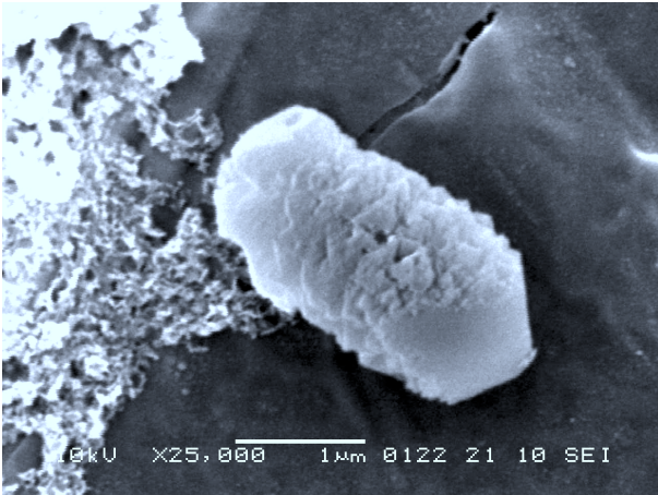
Fig. 3: SEM picture of isolated microcrystal on a Formvar-covered TEM grid. Notice the multilayered structure and sharpen extremities. Sketch of two ( \square:m )T type texture, with or without rotation.
