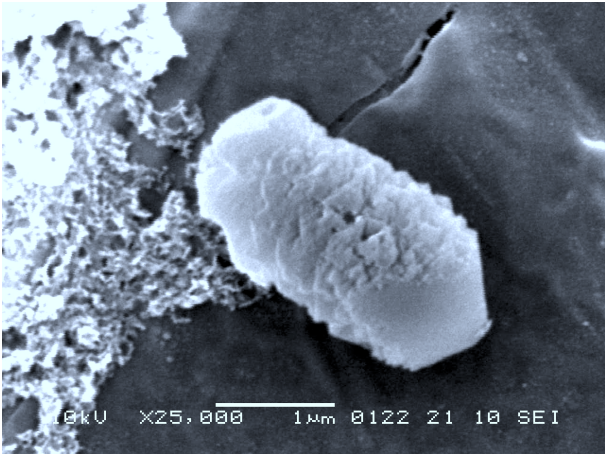
Fig. 3: SEM picture of isolated microcrystal on a Formvar-covered TEM grid. Notice the multilayered structure and sharpened extremities. Sketch of two (□:m)T type texture, with or without rotation.
