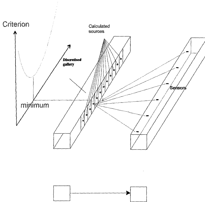
Figure 4: Grid search technique for the detection of trapped miners. A grid size is defined for the calculation of travel times in each pixel. For a velocity model and with the experimental errors, the minimum of the criterion between calculated and observed travel times is chosen as the location of the trapped miners.
