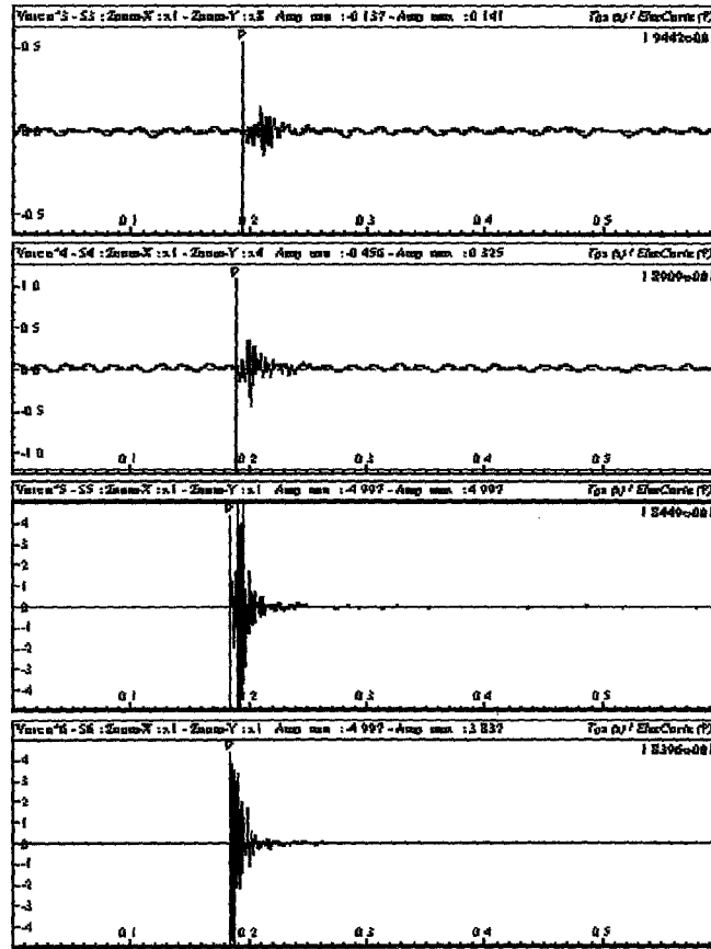
Figure 6: Example of seismic event recorded on four channels at shot point 2 from section E (sidewall facing the rescue team gallery for parallel galleries). The waveforms are 0.6 seconds long with a 15 kHz sampling frequency. The P-wave arrivals have been picked for a grid search location processing.
