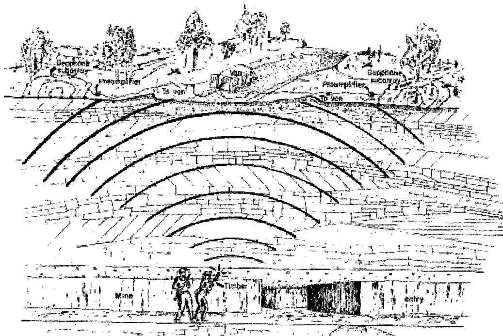
Figure 1 : Detection of trapped miners from a set of geophones deployed from the surface. The miners are hitting the sidewalls of the underground gallery and shot are located from the analysis of P-wave arrival times on the sensors. (from Dobroski and Stolarsczy, 1982).
