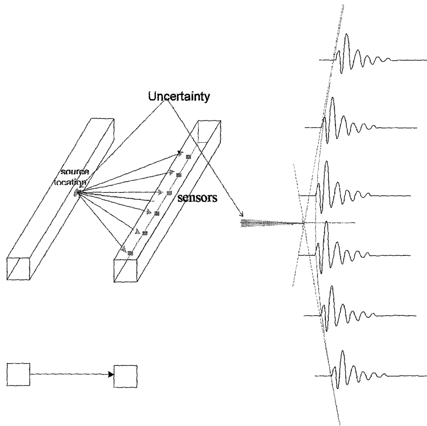
Figure 2: Graphical technique previously used at Charbonnages de France for the detection of trapped miners in a simple configuration. Two lines joining the P wave arrival times are drawn. The intersection of the two lines is indicating the direction and the location of the seismic source. Depending upon the experimental and picking errors, an uncertainty has to be estimated (Grisard et al, 1981).
