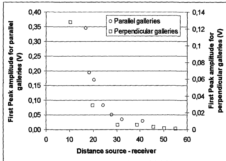
Figure 8: Energy attenuation of a seismic shot as a function of distance to the sensors for a shot recorded in the perpendicular and parallel gallery tests. The large decrease of the energy between 10 and 20 metres in the perpendicular galleries, compared to the parallel galleries, is attributed to a significantly damaged rock mass.
