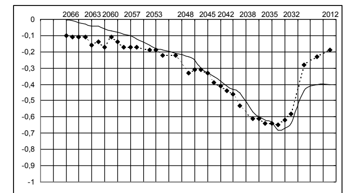
Fig. 4. Measured (diamonds) and calculated (solid line) subsidence along the path of observations in the mine Estaque Sud in the Provence coal district of France
