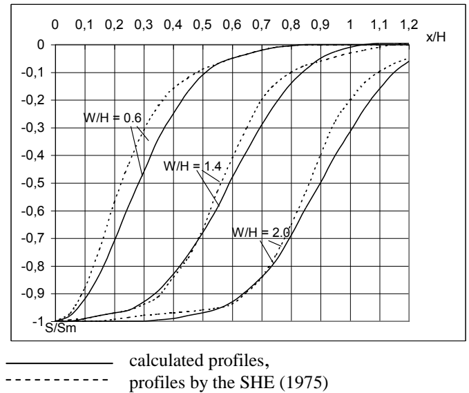
Fig. 2. Profiles of subsidence for sub-critical ( L/W=0.6 ), critical ( L/W=1.4 ) and super-critical ( L/W=2.0 ) areas
