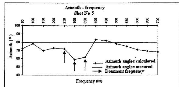
Figure 10 : Unfavourable case in which the azimuth is not associated with the dominant frequencies..
